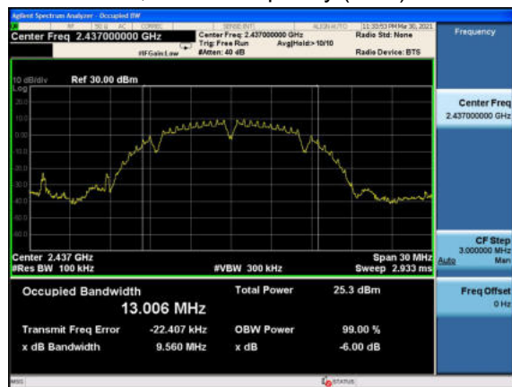
802.11b, Carrier frequency (MHz): 2437
