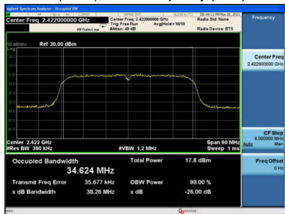
802.11n(HT40), Carrier frequency (MHz): 2422
