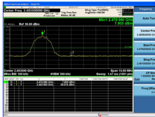
Bluetooth LE (2M), Channel No.: 39
