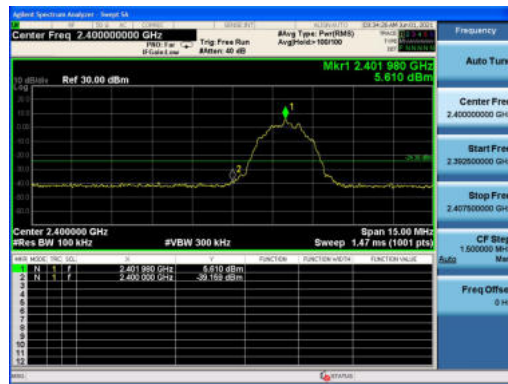
Bluetooth LE (2M), Channel No.: 0
