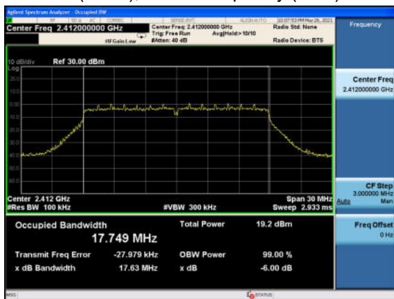
802.11n(HT20), Carrier frequency (MHz): 2412
