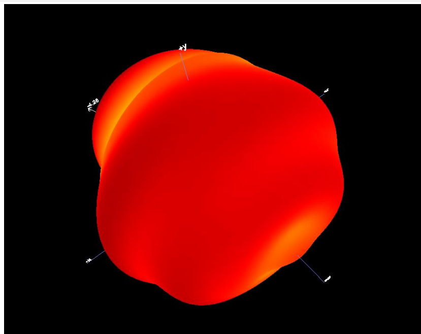
B1.2 3D Pattern for 908.42MHz
