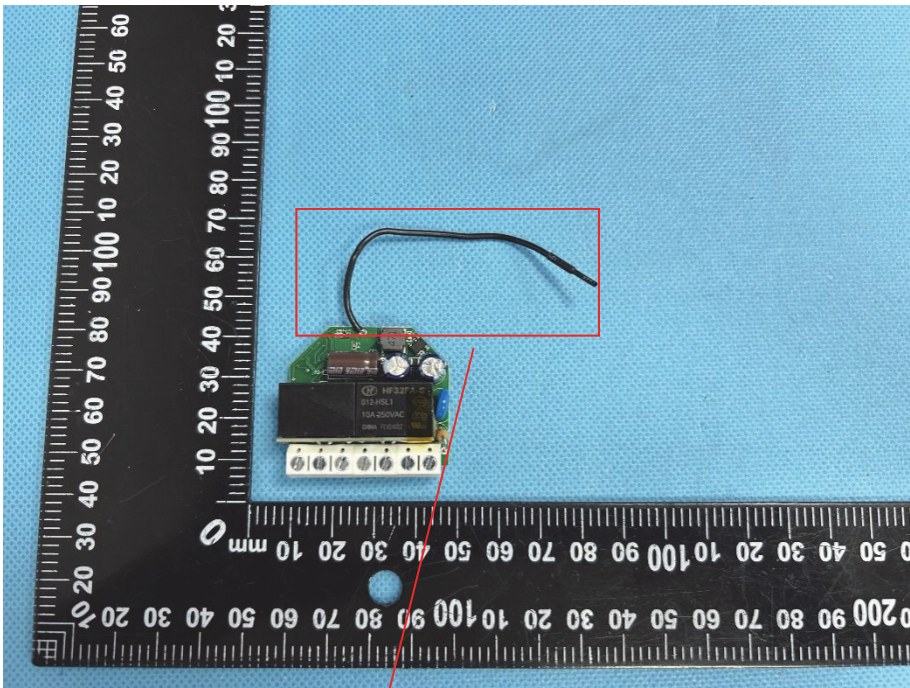
Z-Wave Ant.
