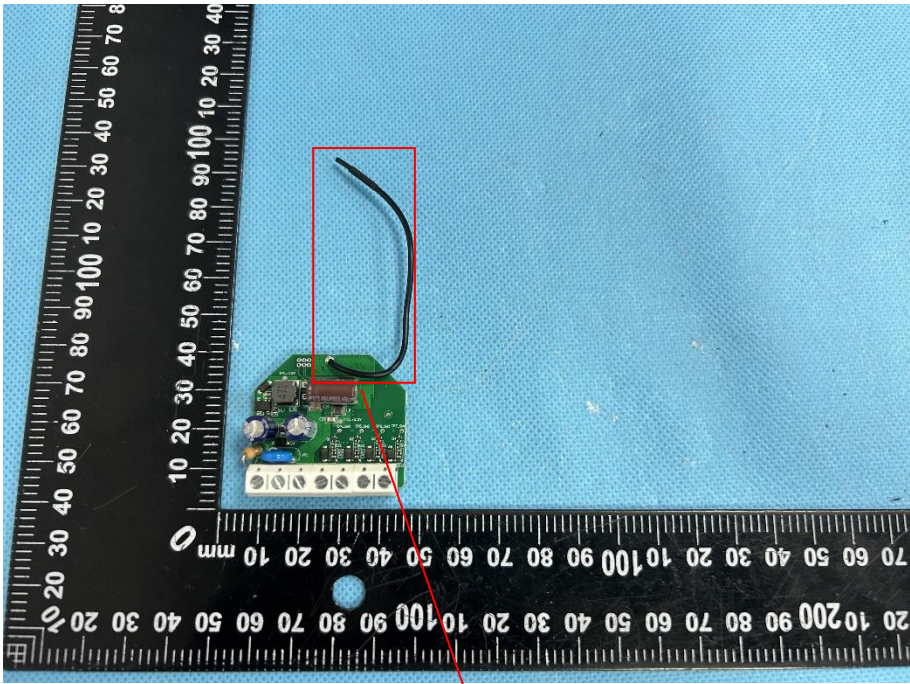
Z-Wave Ant.
