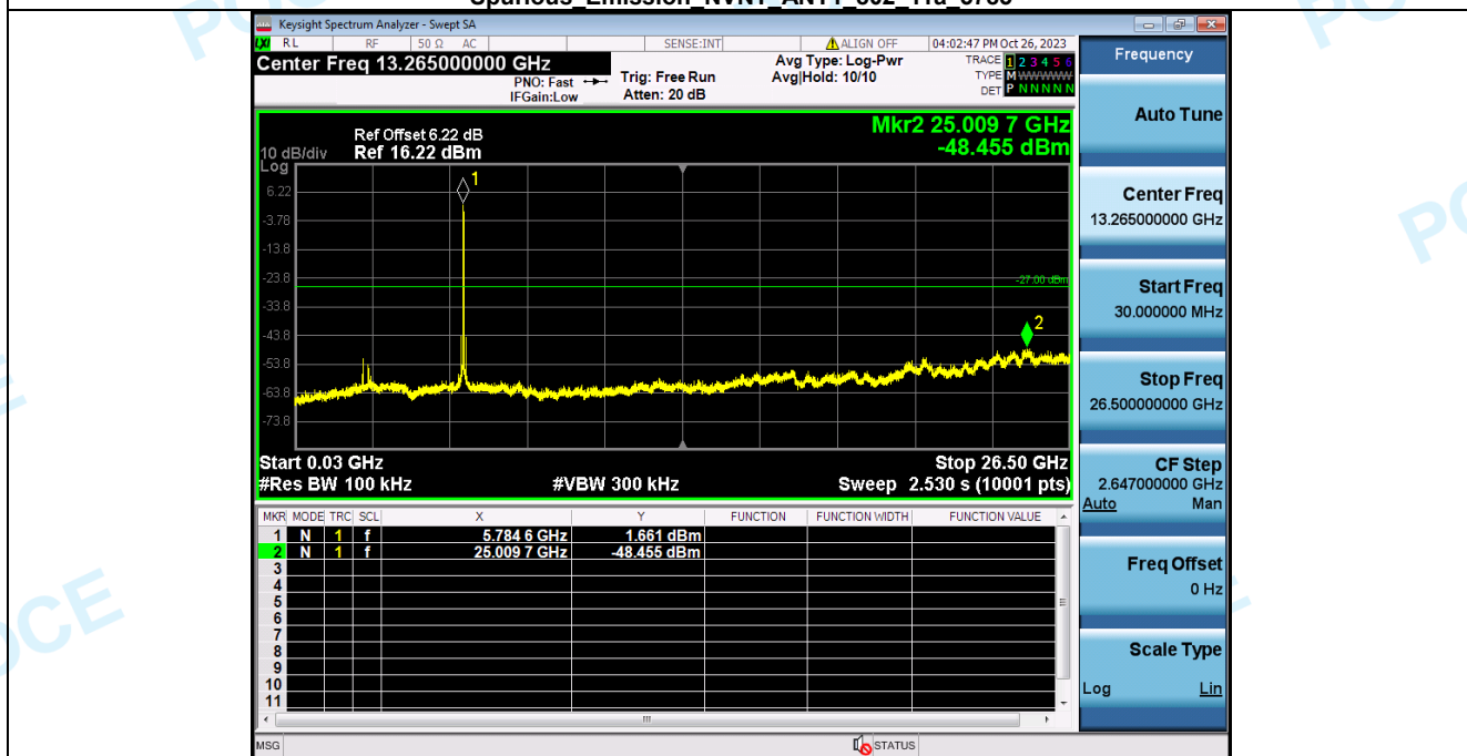
Spurious Emission NVNT ANT1 802 11a 5785
