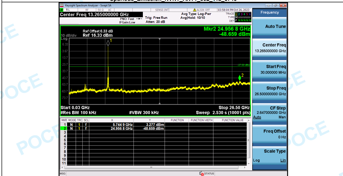
Spurious Emission NVNT ANT1 802 11a 5745
