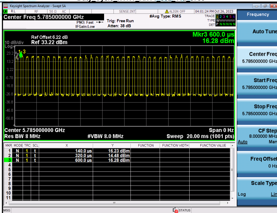
Duty Cycle_NVNT_ANT1_802_11a_5785
