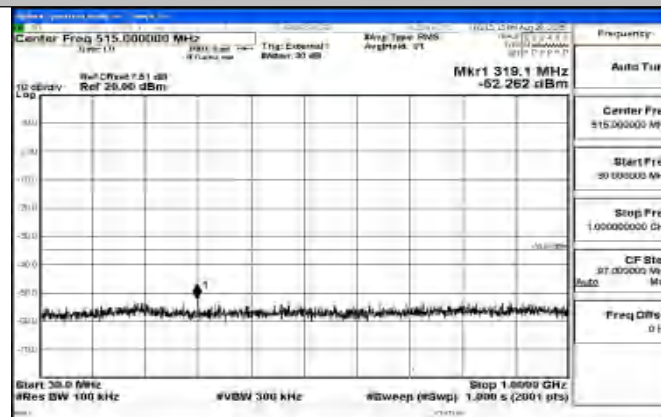
Band41_20MHz_16QAM_41490_1RB#0_30~1000_30~1000
