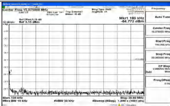
Band41_10MHz_16QAM_39700_1RB#0_0.15~30_0.15~30
