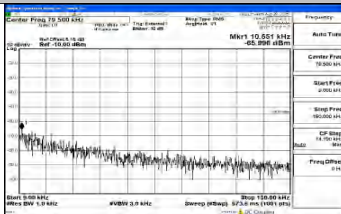
Band41_20MHz_QPSK_41490_1RB#0_0.009~0.15_0.009~0.15
