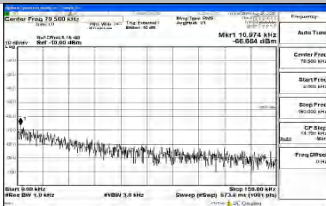
Band41_20MHz_QPSK_39750_1RB#0_0.009~0.15_0.009~0.15
