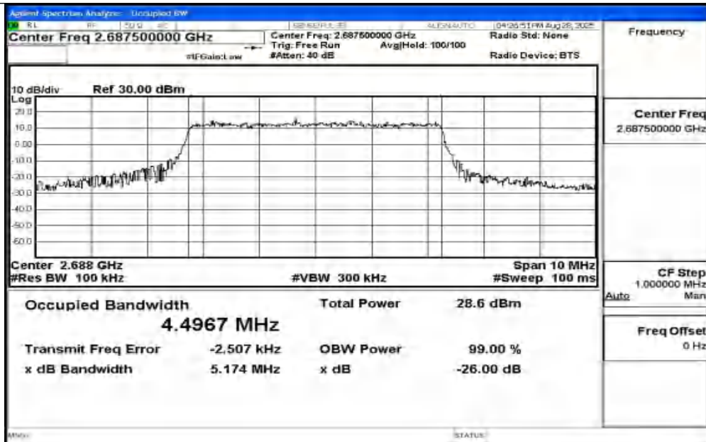
Band41-5MHz-QPSK-41565-25RB#0-PASS
