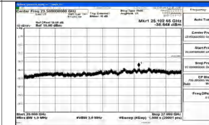
Band41_5MHz_16QAM_39675_1RB#0_20000~27000_20000~ 00
