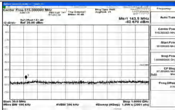
Band41_20MHz_QPSK_41490_1RB#0_30~1000_30~1000
