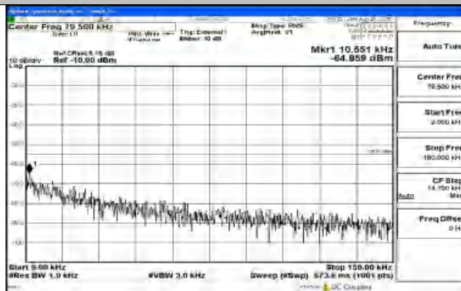
Band41_10MHz_QPSK_39700_1RB#0_0.009~0.15_0.009~0.15
