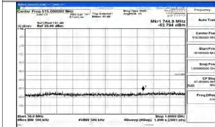
Band41_5MHz_QPSK_39675_1RB#0_30~1000_30~1000
