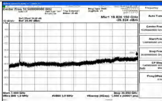
Band41_20MHz_16QAM_40620_1RB#0_1000~20000_1000~2000
