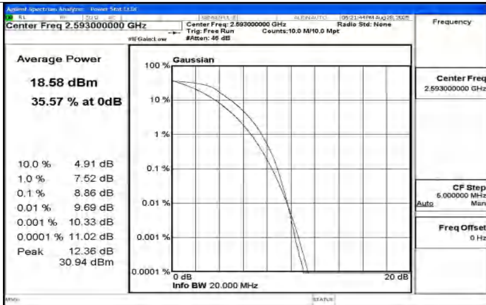
Band41-20MHz-QPSK-40620-100RB#0-PASS
