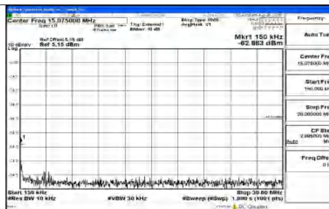
Band41_15MHz_QPSK_41515_1RB#0_0.15~30_0.15~30
