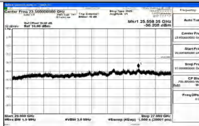
Band41_15MHz_16QAM_40620_1RB#0_20000~27000_20000~27000
