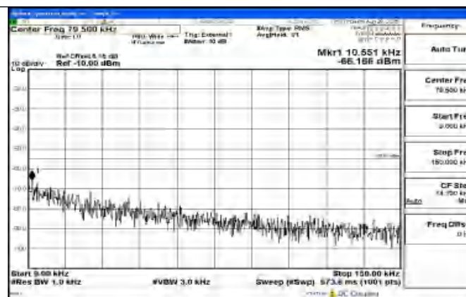
Band41_10MHz_16QAM_39700_1RB#0_0.009~0.15_0.009~0.15
