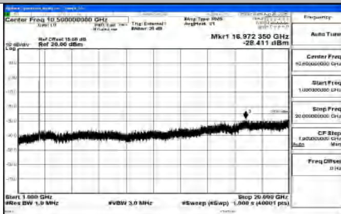
Band41_10MHz_16QAM_39700_1RB#0_1000~20000_1000~2000
