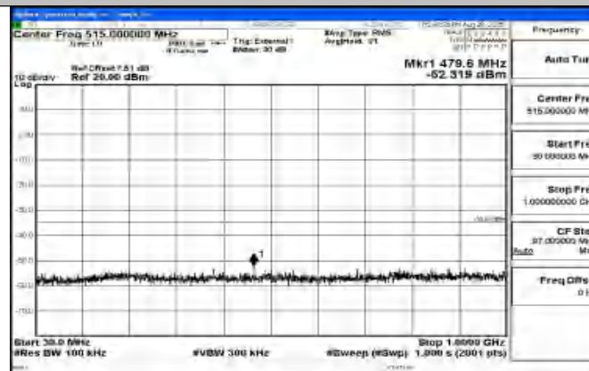
Band41_15MHz_16QAM_40620_1RB#0_30~1000_30~1000
