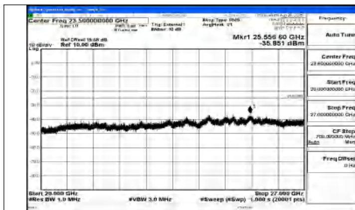
Band41_10MHz_QPSK_39700_1RB#0_20000~27000_20000~27000
