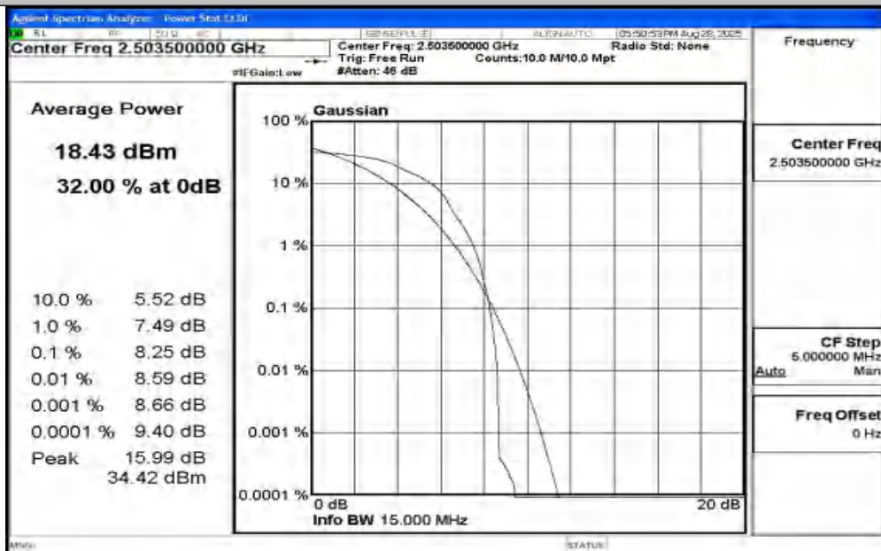
Band41-15MHz-16QAM-39725-1RB#0-PASS
