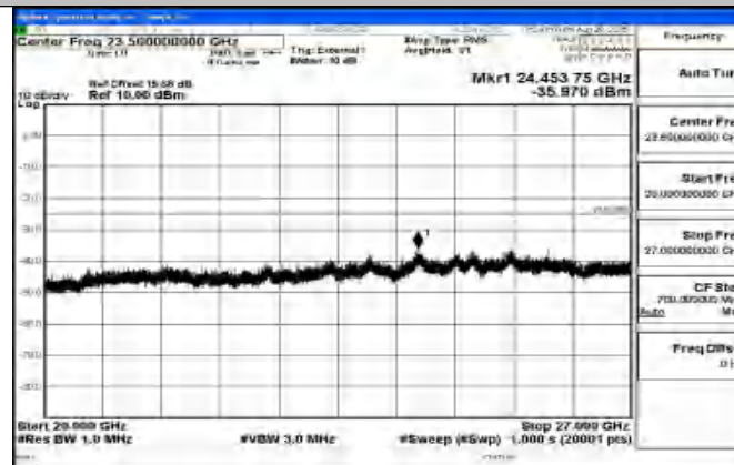
Band41_15MHz_16QAM_41515_1RB#0_20000~27000_20000~27000
