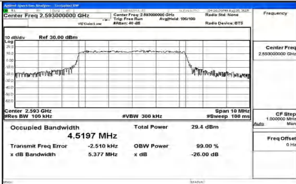
Band41-5MHz-16QAM-40620-25RB#0-PASS
