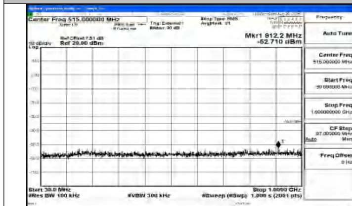
Band41_20MHz_QPSK_40620_1RB#0_30~1000_30~1000
