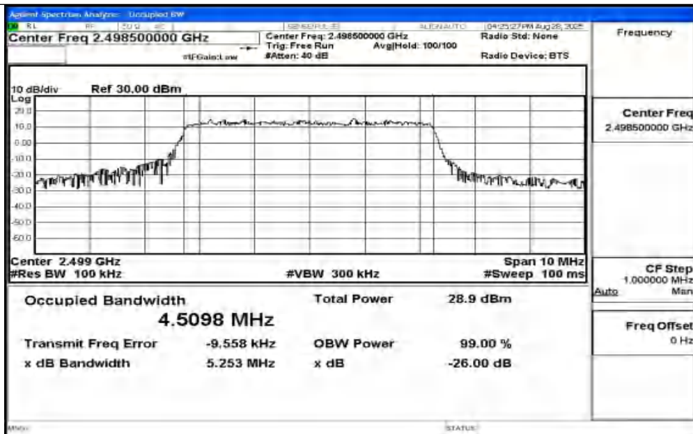
Band41-5MHz-QPSK-39675-25RB#0-PASS
