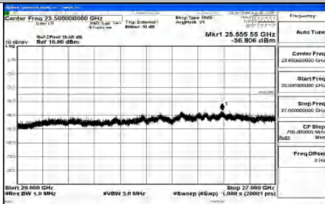
Band41_5MHz_QPSK_41565_1RB#0_20000~27000_20000~27000
