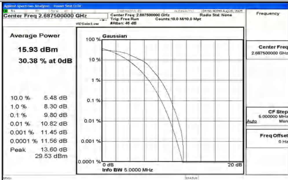
Band41-5MHz-16QAM-41565-25RB#0-PASS
