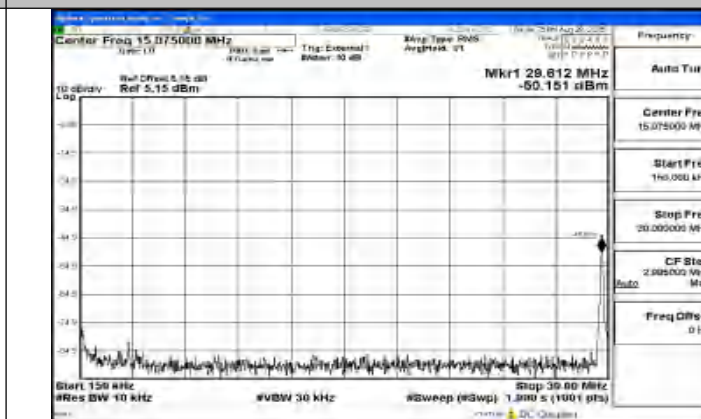
Band41_5MHz_QPSK_40620_1RB#0_0.15~30_0.15~30
