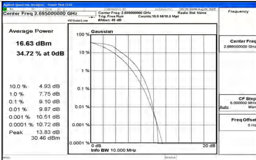
Band41-10MHz-QPSK-41540-50RB#0-PASS
