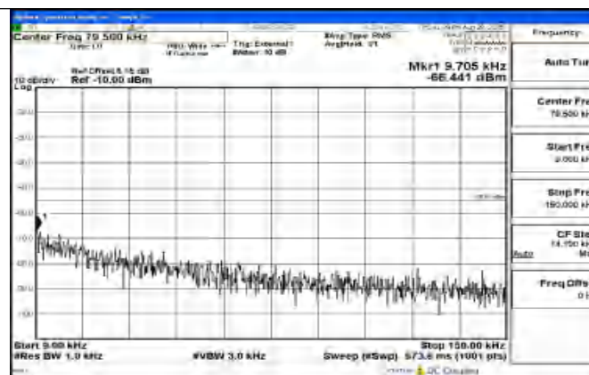
Band41_15MHz_16QAM_40620_1RB#0_0.009~0.15_0.009~0.15
