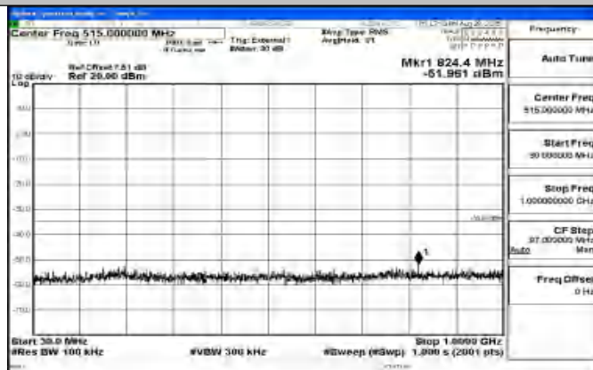
Band41_10MHz_QPSK_41540_1RB#0_30~1000_30~1000
