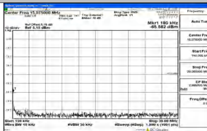
Band41_10MHz_QPSK_41540_1RB#0_0.15~30_0.15~30
