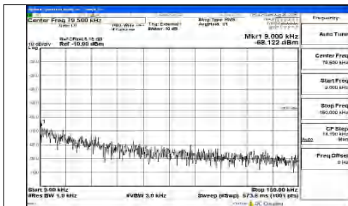
Band41_15MHz_QPSK_41515_1RB#0_0.009~0.15_0.009~0.15
