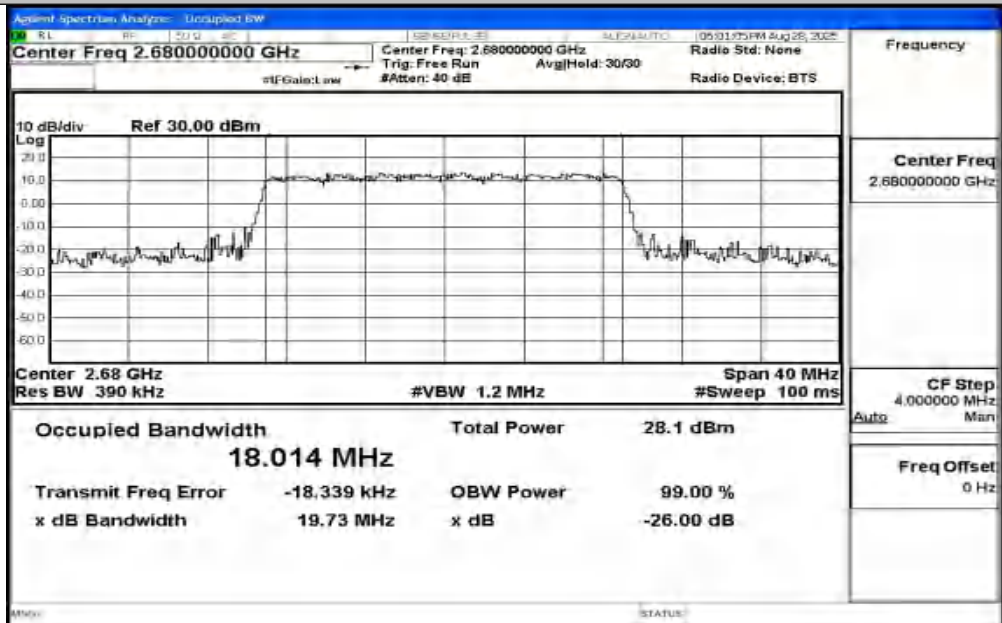
Band41-20MHz-16QAM-41490-100RB#0-PASS
