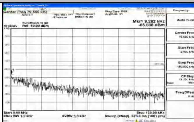
Band41_15MHz_QPSK_40620_1RB#0_0.009~0.15_0.009~0.15
