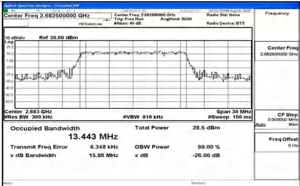
Band41-15MHz-QPSK-41515-75RB#0-PASS
