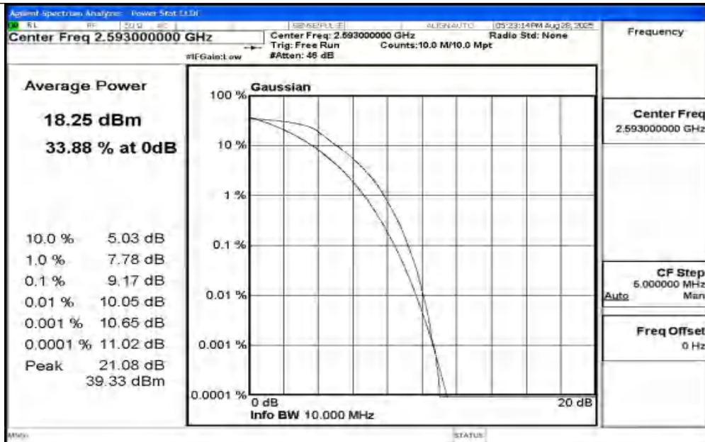
Band41-10MHz-QPSK-40620-50RB#0-PASS
