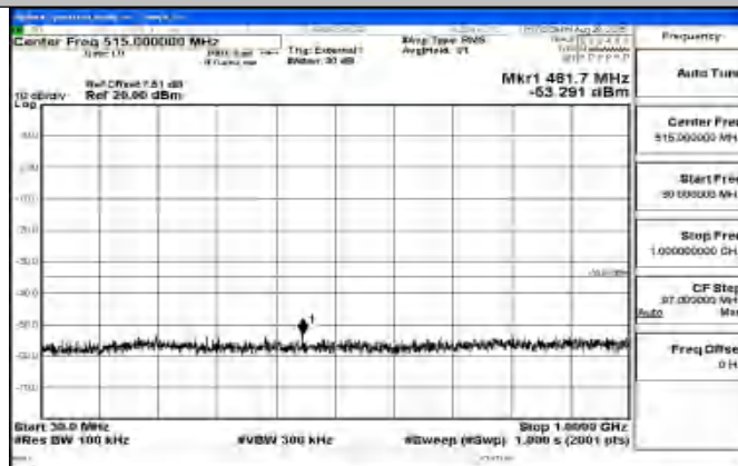
Band41_10MHz_QPSK_39700_1RB#0_30~1000_30~1000
