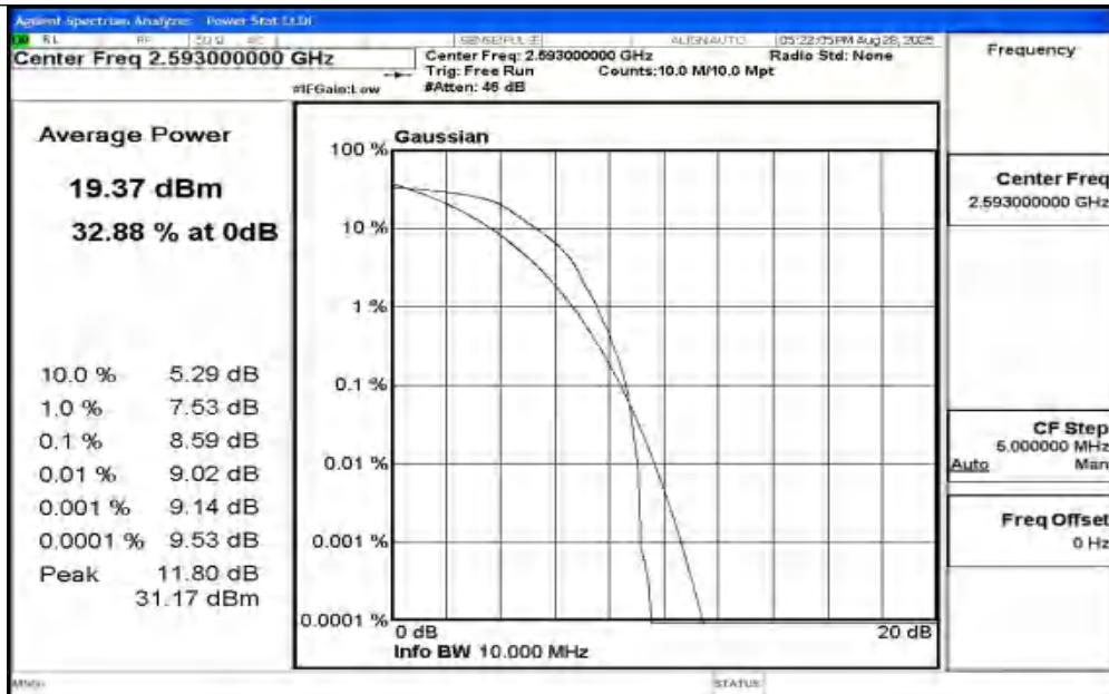
Band41-10MHz-QPSK-40620-1RB#0-PASS
