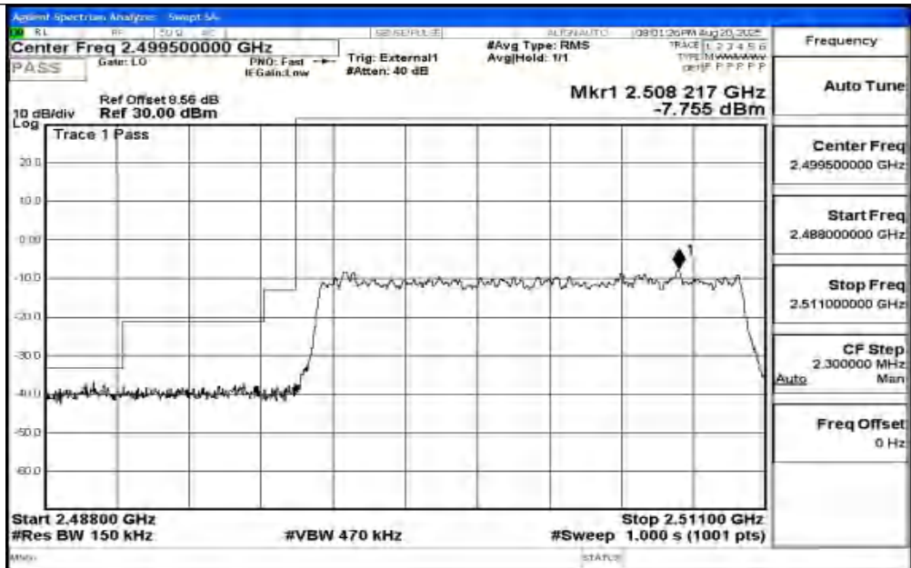
Band41_15MHz_16QAM_39725_75RB#0
