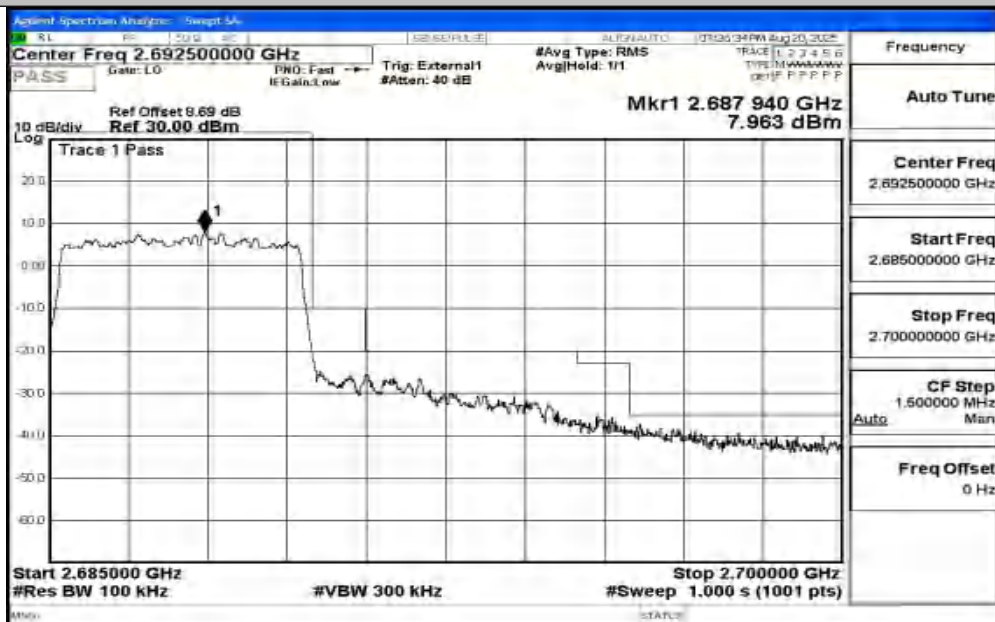
Band41_5MHz_16QAM_41565_25RB#0
