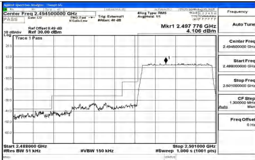
Band41_5MHz_QPSK_39675_25RB#0
