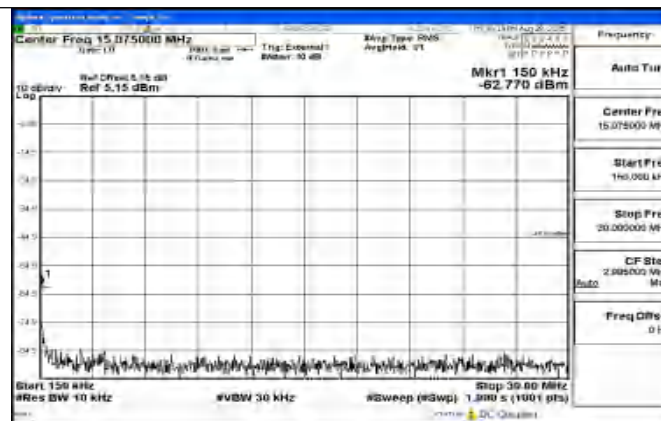
Band41_15MHz_QPSK_39725_1RB#0_0.15~30_0.15~30
