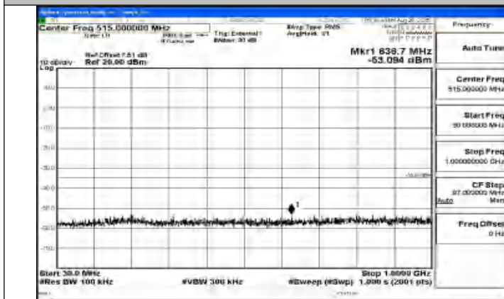
Band41_15MHz_QPSK_39725_1RB#0_30~1000_30~1000
