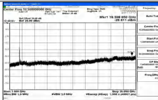
Band41_15MHz_QPSK_39725_1RB#0_1000~20000_1000~20000
