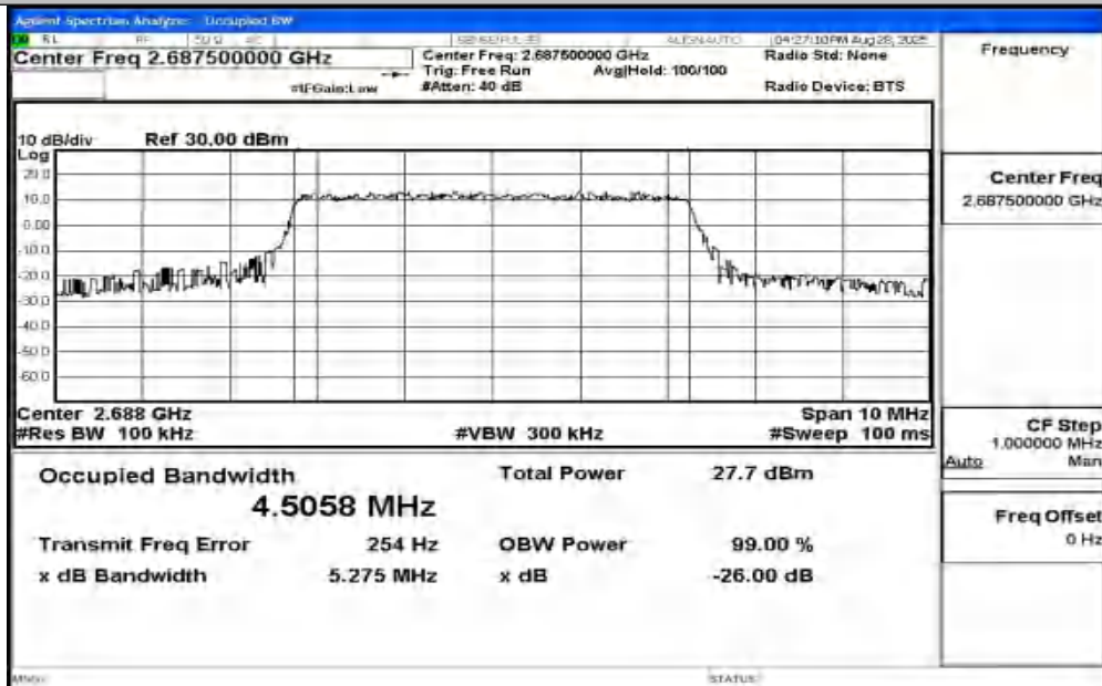
Band41-5MHz-16QAM-41565-25RB#0-PASS
