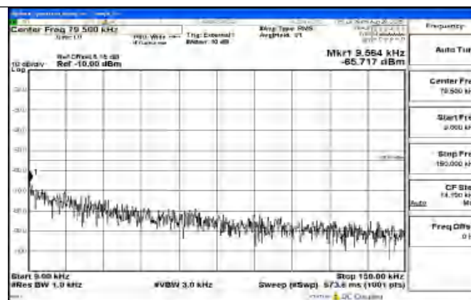
Band41_10MHz_16QAM_41540_1RB#0_0.009~0.15_0.009~0.15
