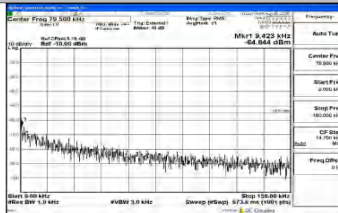
Band41_20MHz_16QAM_40620_1RB#0_0.009~0.15_0.009~0.15
