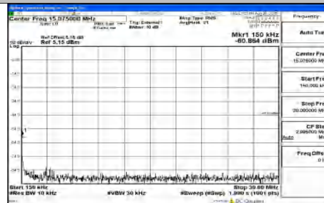
Band41_20MHz_QPSK_41490_1RB#0_0.15~30_0.15~30
