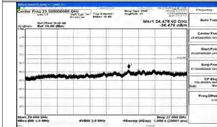
Band41_5MHz_QPSK_39675_1RB#0_20000~27000_20000~27000
