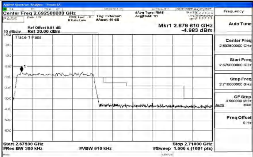
Band41_15MHz_16QAM_41515_75RB#0
