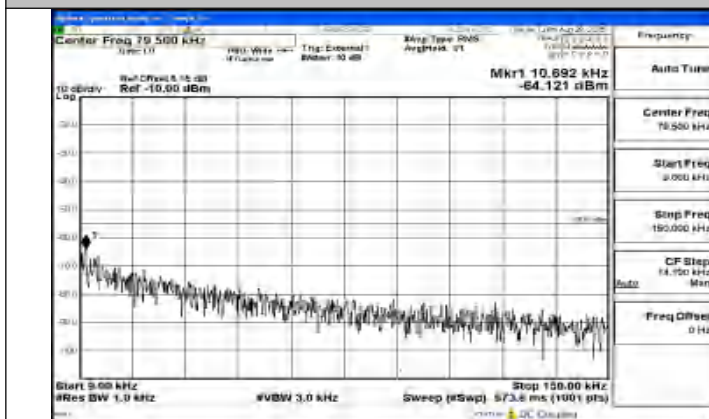
Band41_5MHz_QPSK_40620_1RB#0_0.009~0.15_0.009~0.15
