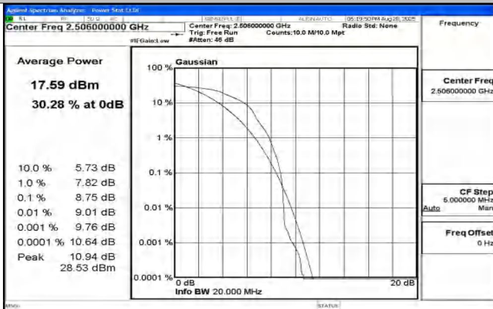
Band41-20MHz-16QAM-39750-1RB#0-PASS
