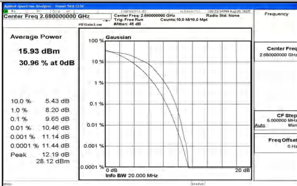
Band41-20MHz-16QAM-41490-100RB#0-PASS
