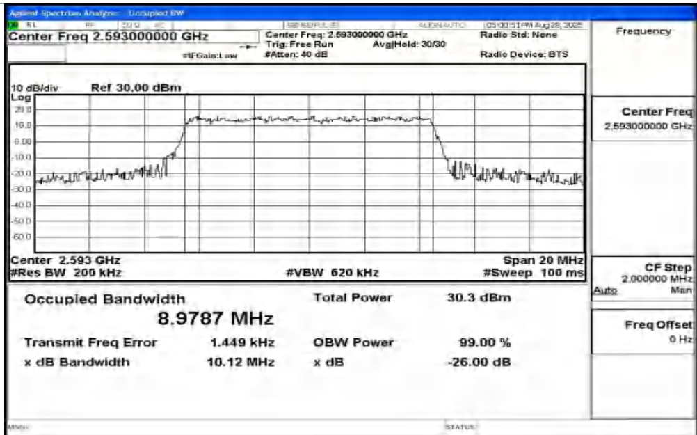
Band41-10MHz-QPSK-40620-50RB#0-PASS
