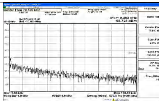
Band41_20MHz_16QAM_39750_1RB#0_0.009~0.15_0.009~0.15
