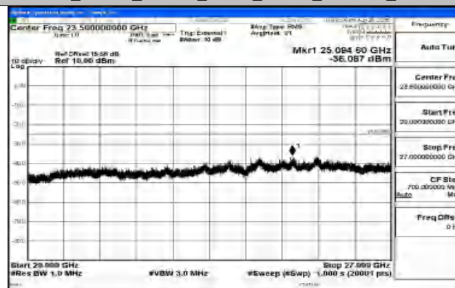
Band41_20MHz_16QAM_39750_1RB#0_20000~27000_20000~27000
