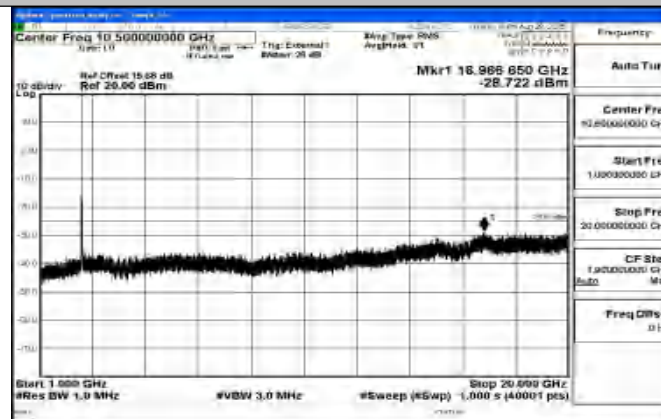
Band41_20MHz_QPSK_39750_1RB#0_1000~20000_1000~20000
