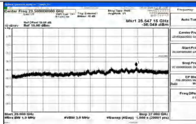
Band41_15MHz_16QAM_39725_1RB#0_20000~27000_20000~27000
