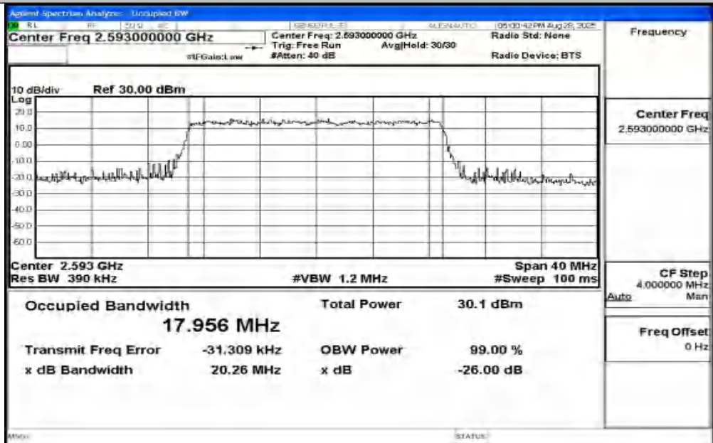
Band41-20MHz-16QAM-40620-100RB#0-PASS
