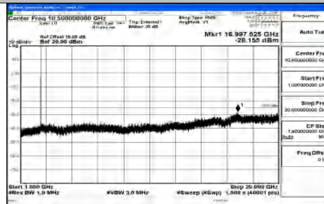
Band41_10MHz_QPSK_39700_1RB#0_1000~20000_1000~20000
