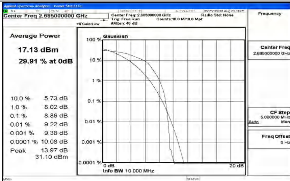
Band41-10MHz-16QAM-41540-1RB#0-PASS
