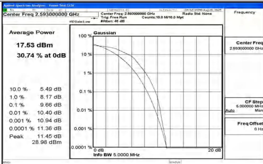
Band41-5MHz-16QAM-40620-25RB#0-PASS
