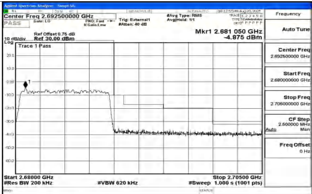
Band41_10MHz_16QAM_41540_50RB#0
