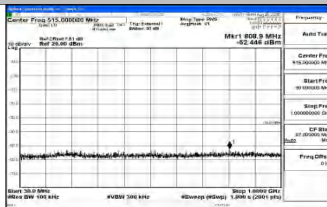
Band41_20MHz_16QAM_39750_1RB#0_30~1000_30~1000
