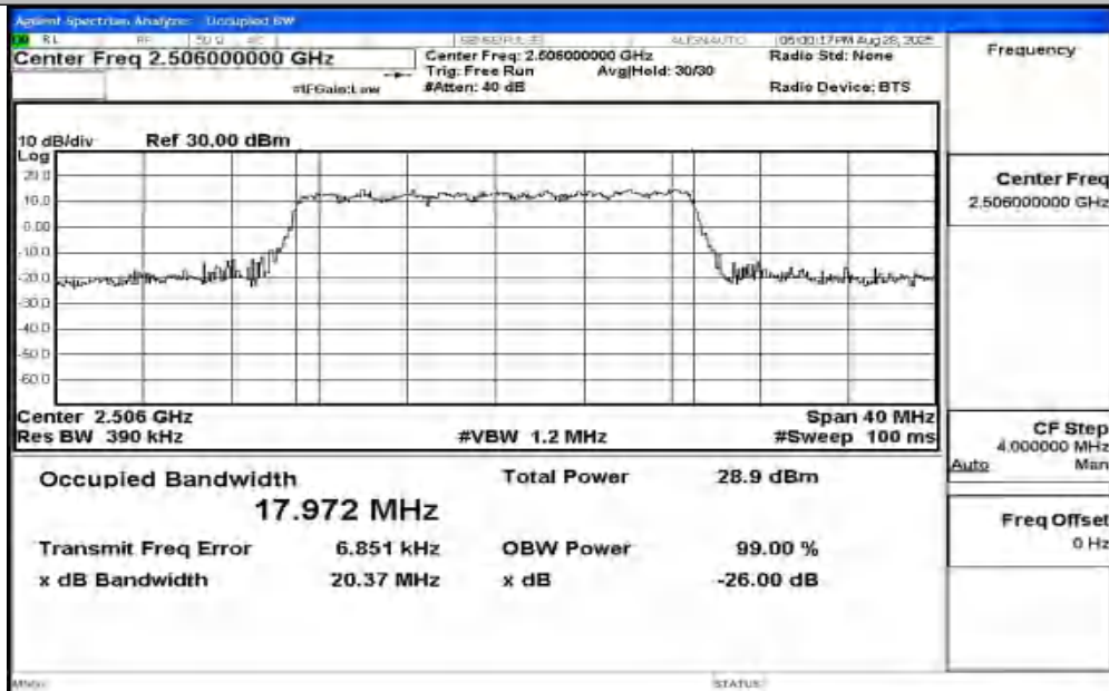
Band41-20MHz-16QAM-39750-100RB#0-PASS
