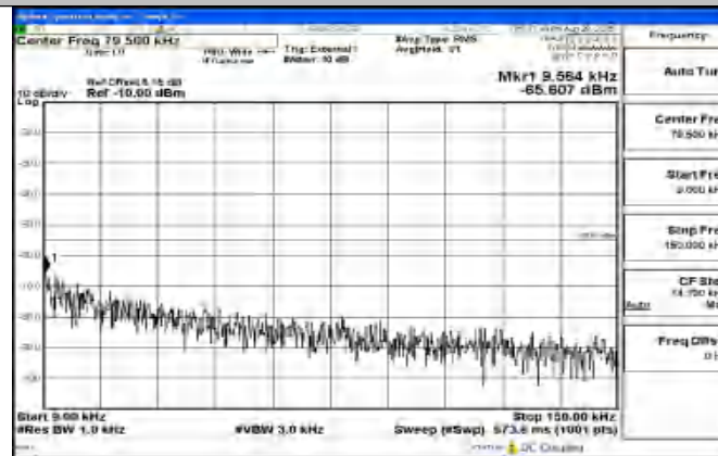
Band41_15MHz_16QAM_39725_1RB#0_0.009~0.15_0.009~0.15
