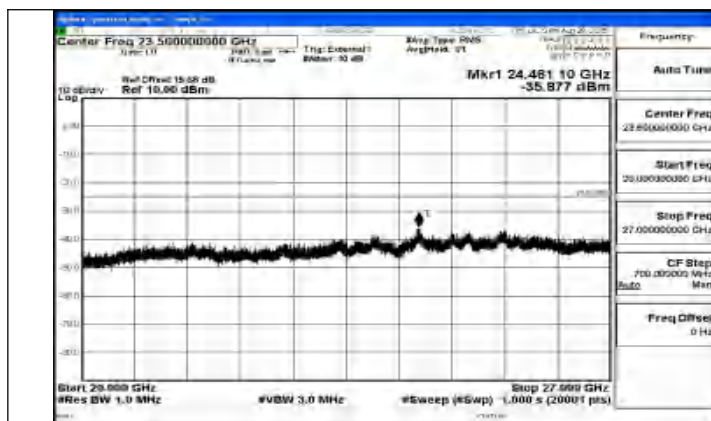
Band41_10MHz_QPSK_41540_1RB#0_20000~27000_20000~27000
