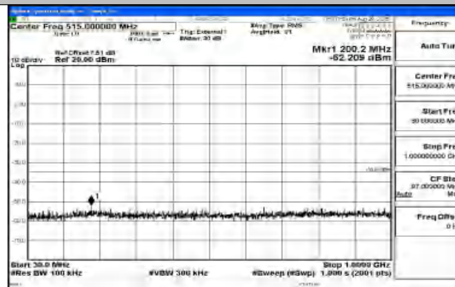
Band41_10MHz_16QAM_39700_1RB#0_30~1000_30~1000
