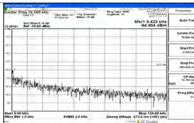
Band41_20MHz_16QAM_41490_1RB#0_0.009~0.15_0.009~0.15
