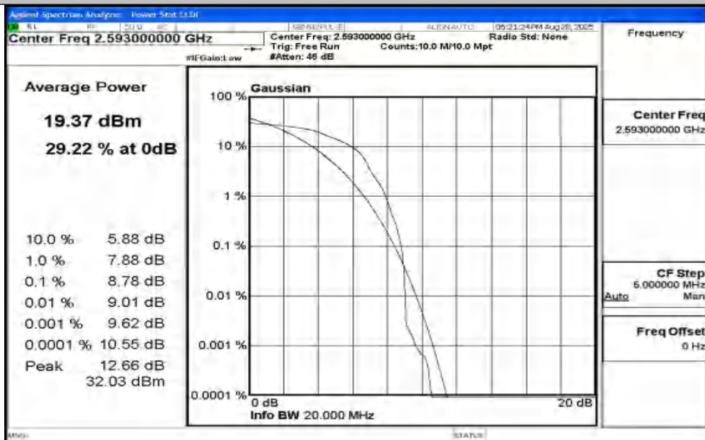
Band41-20MHz-16QAM-40620-1RB#0-PASS
