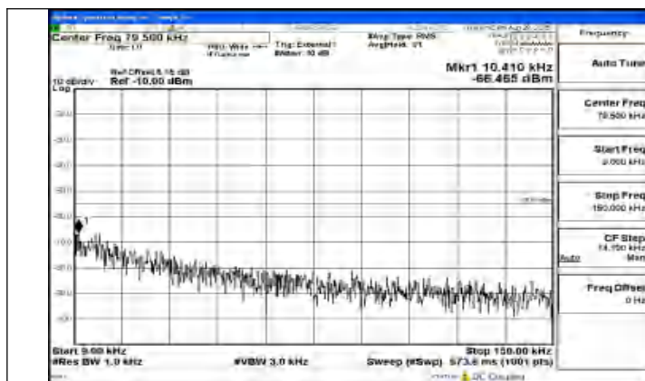
Band41_20MHz_QPSK_40620_1RB#0_0.009~0.15_0.009~0.15
