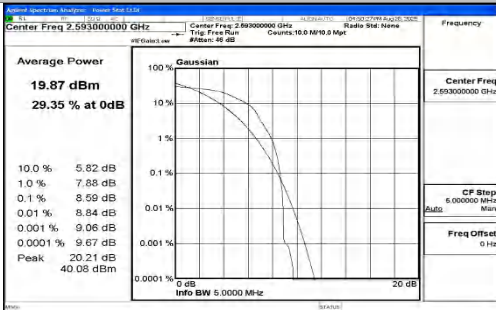
Band41-5MHz-16QAM-40620-1RB#0-PASS
