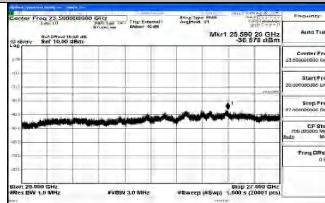
Band41_20MHz_16QAM_40620_1RB#0_20000~27000_20000~20000
