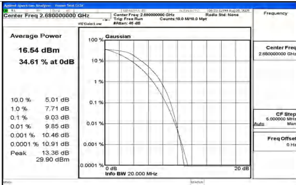
Band41-20MHz-QPSK-41490-100RB#0-PASS
