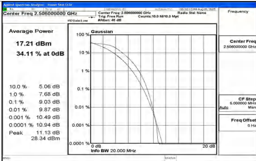
Band41-20MHz-QPSK-39750-100RB#0-PASS
