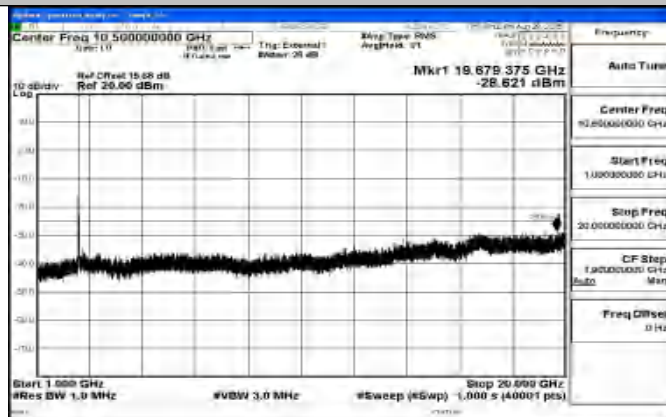
Band41_15MHz_16QAM_39725_1RB#0_1000~20000_1000~2000
