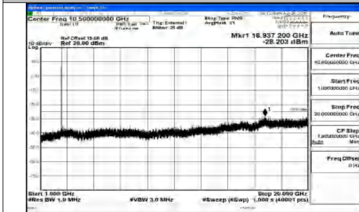
Band41_5MHz_16QAM_39675_1RB#0_1000~20000_1000~20000
