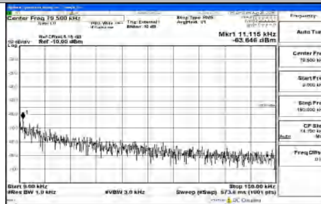
Band41_10MHz_16QAM_40620_1RB#0_0.009~0.15_0.009~0.15
