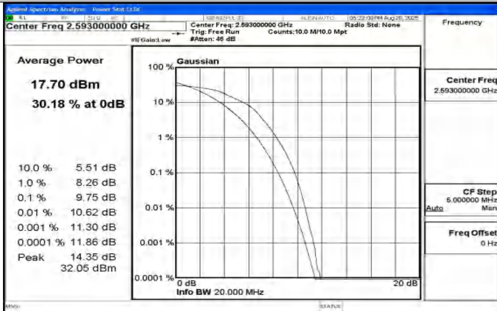
Band41-20MHz-16QAM-40620-100RB#0-PASS
