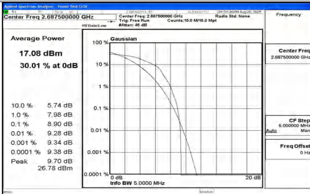
Band41-5MHz-16QAM-41565-1RB#0-PASS
