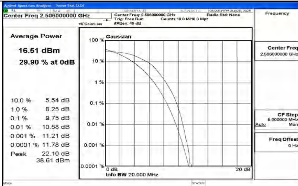
Band41-20MHz-16QAM-39750-100RB#0-PASS
