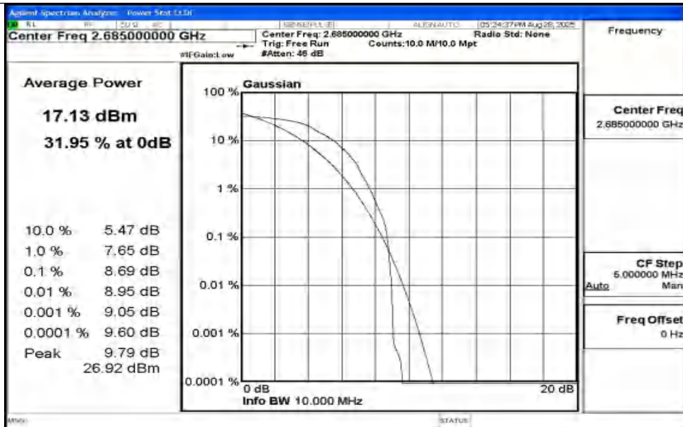
Band41-10MHz-QPSK-41540-1RB#0-PASS
