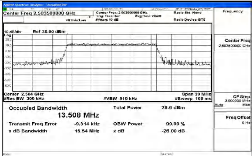
Band41-15MHz-16QAM-39725-75RB#0-PASS
