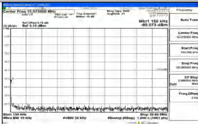
Band41_20MHz_16QAM_41490_1RB#0_0.15~30_0.15~30
