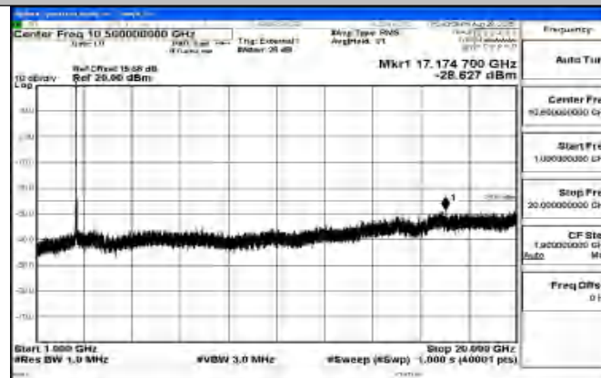
Band41_15MHz_QPSK_40620_1RB#0_1000~20000_1000~20000
