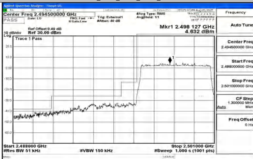
Band41_5MHz_16QAM_39675_25RB#0
