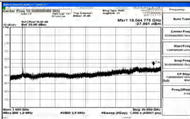
Band41_15MHz_16QAM_40620_1RB#0_1000~20000_1000~20000
