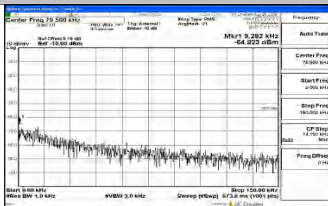
Band41_10MHz_QPSK_41540_1RB#0_0.009~0.15_0.009~0.15
