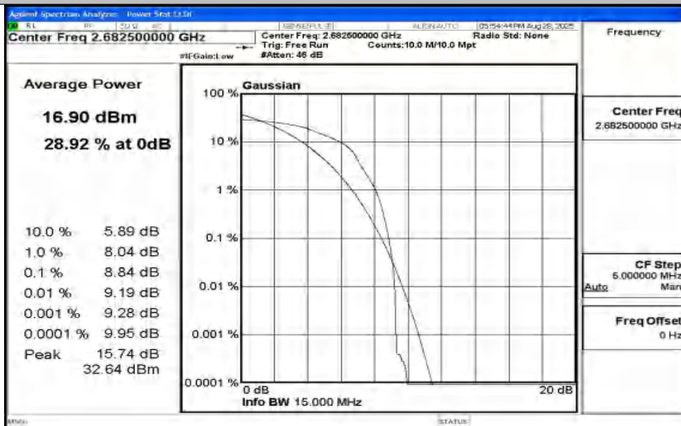
Band41-15MHz-16QAM-41515-1RB#0-PASS
