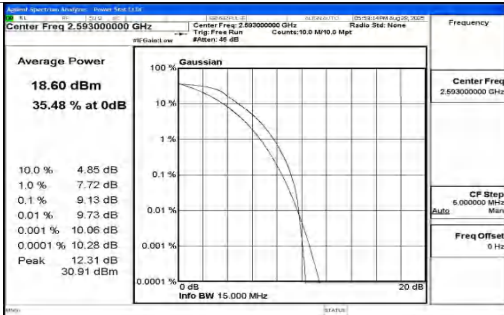
Band41-15MHz-QPSK-40620-75RB#0-PASS
