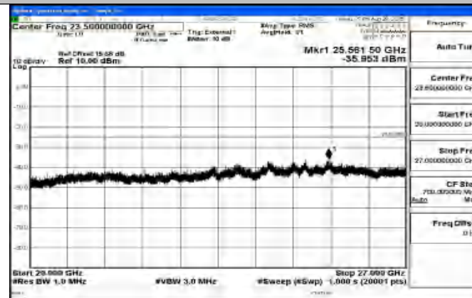
Band41_5MHz_16QAM_41565_1RB#0_20000~27000_20000~27000
