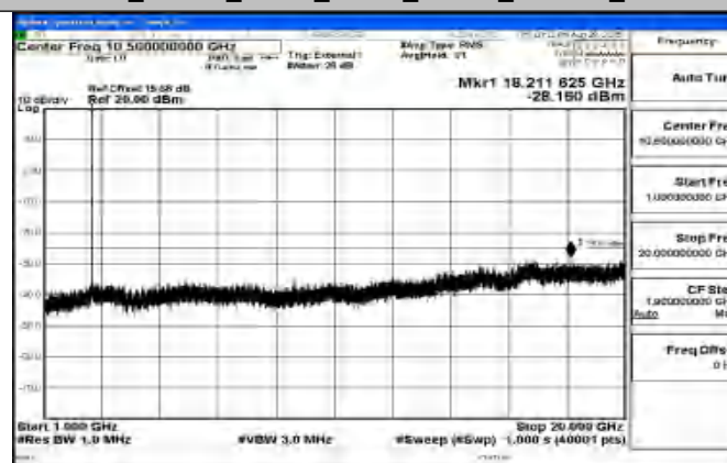
Band41_10MHz_QPSK_40620_1RB#0_1000~20000_1000~20000
