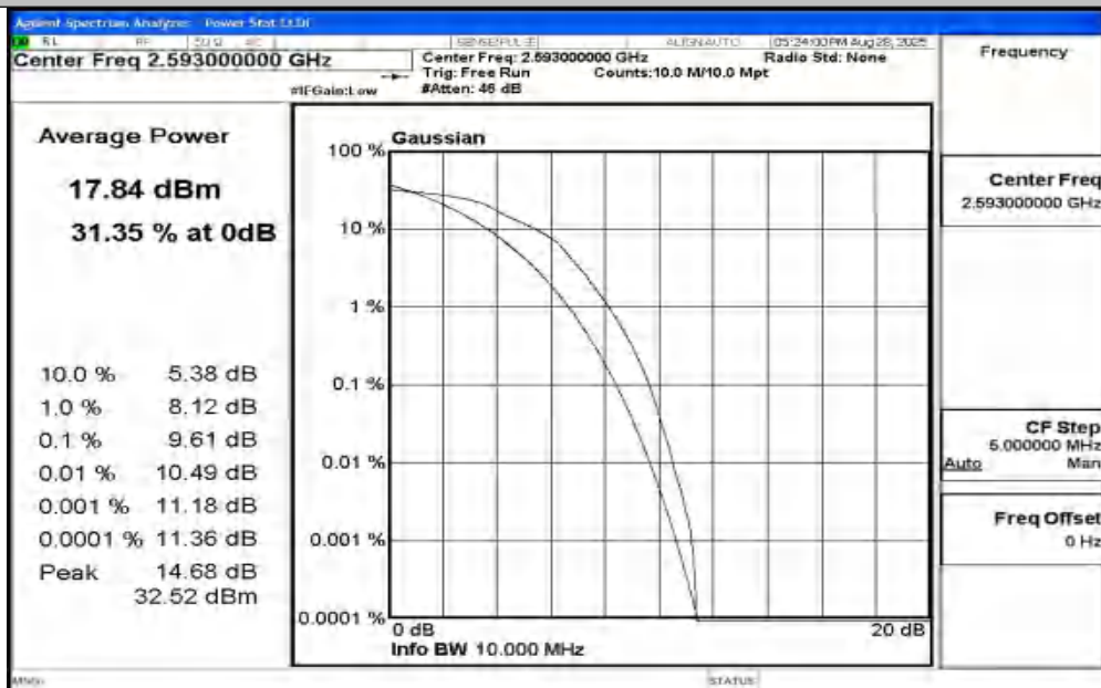
Band41-10MHz-16QAM-40620-50RB#0-PASS
