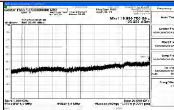
Band41_5MHz_QPSK_39675_1RB#0_1000~20000_1000~20000
