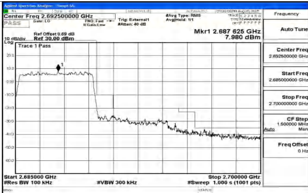
Band41_5MHz_QPSK_41565_25RB#0
