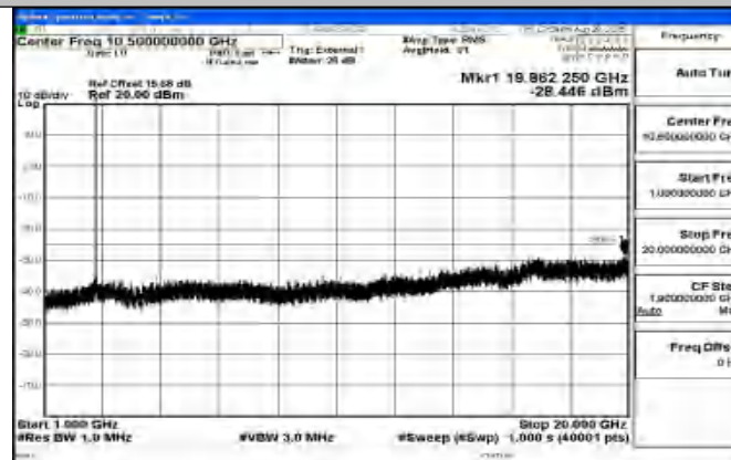
Band41_10MHz_QPSK_41540_1RB#0_1000~20000_1000~20000
