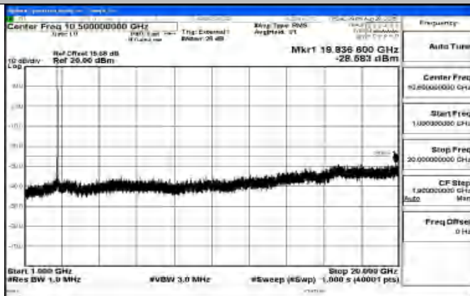
Band41_15MHz_16QAM_41515_1RB#0_1000~20000_1000~2000
