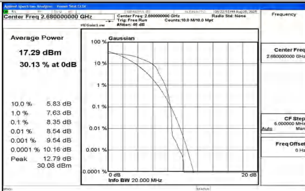
Band41-20MHz-16QAM-41490-1RB#0-PASS
