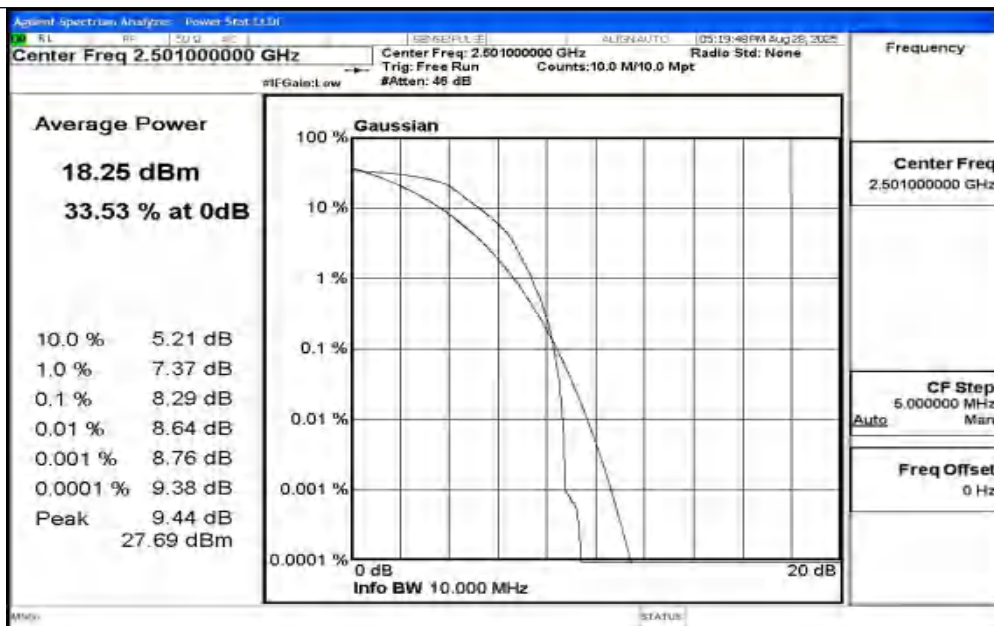
Band41-10MHz-QPSK-39700-1RB#0-PASS
