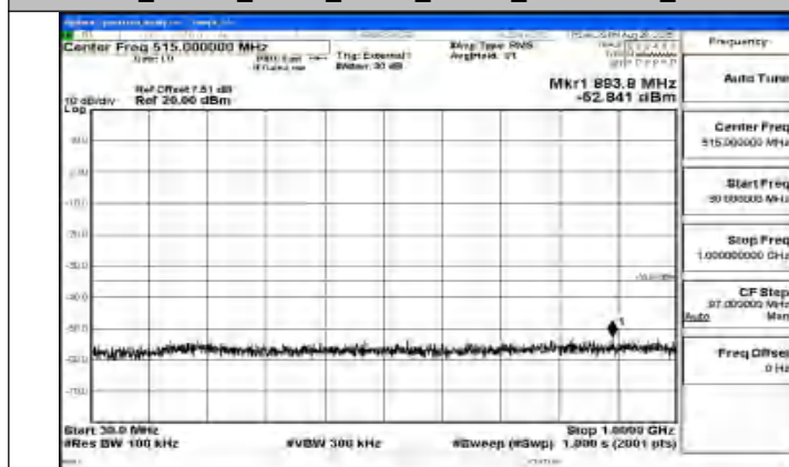
Band41_15MHz_QPSK_41515_1RB#0_30~1000_30~1000
