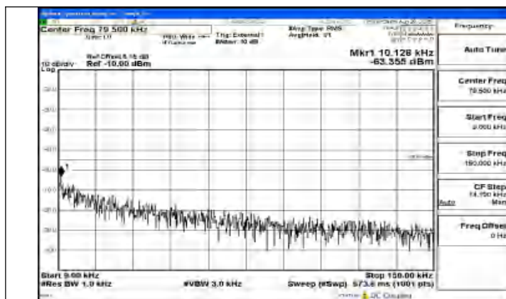
Band41_10MHz_QPSK_40620_1RB#0_0.009~0.15_0.009~0.15
