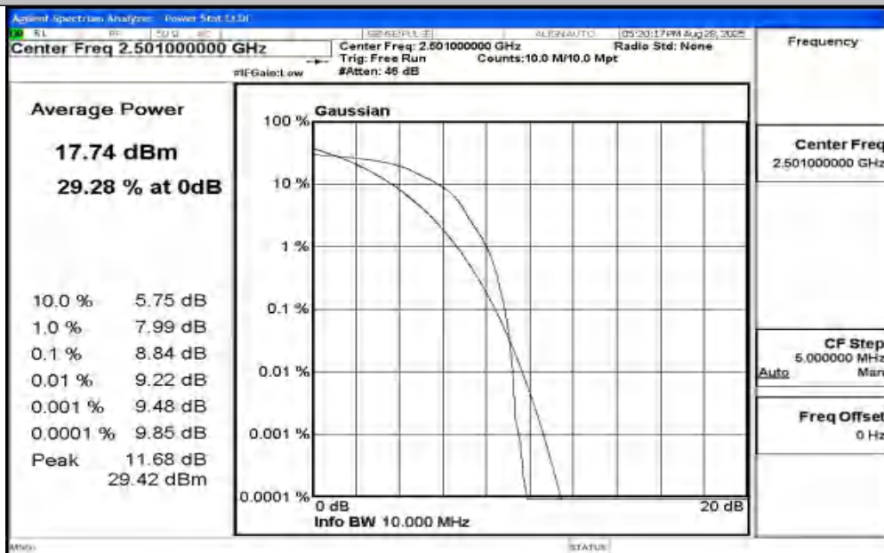
Band41-10MHz-16QAM-39700-1RB#0-PASS
