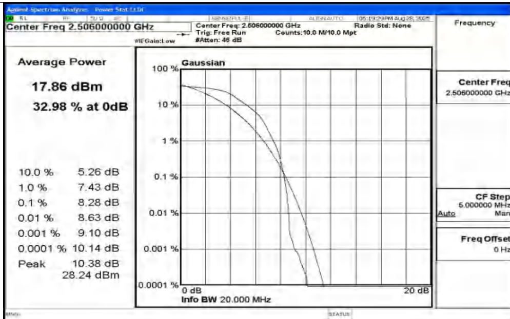
Band41-20MHz-QPSK-39750-1RB#0-PASS
