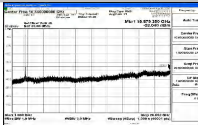
Band41_20MHz_QPSK_40620_1RB#0_1000~20000_1000~20000
