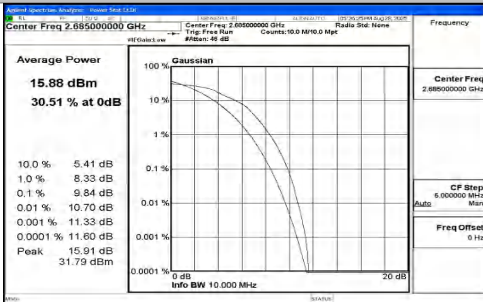
Band41-10MHz-16QAM-41540-50RB#0-PASS
