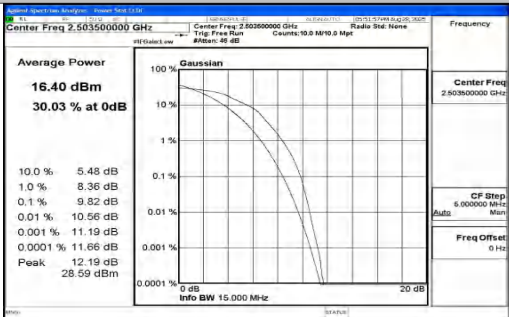
Band41-15MHz-16QAM-39725-75RB#0-PASS
