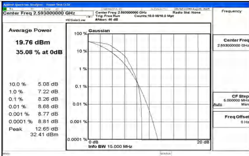
Band41-15MHz-QPSK-40620-1RB#0-PASS
