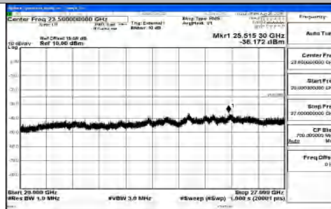
Band41_20MHz_16QAM_41490_1RB#0_20000~27000_20000~27000
