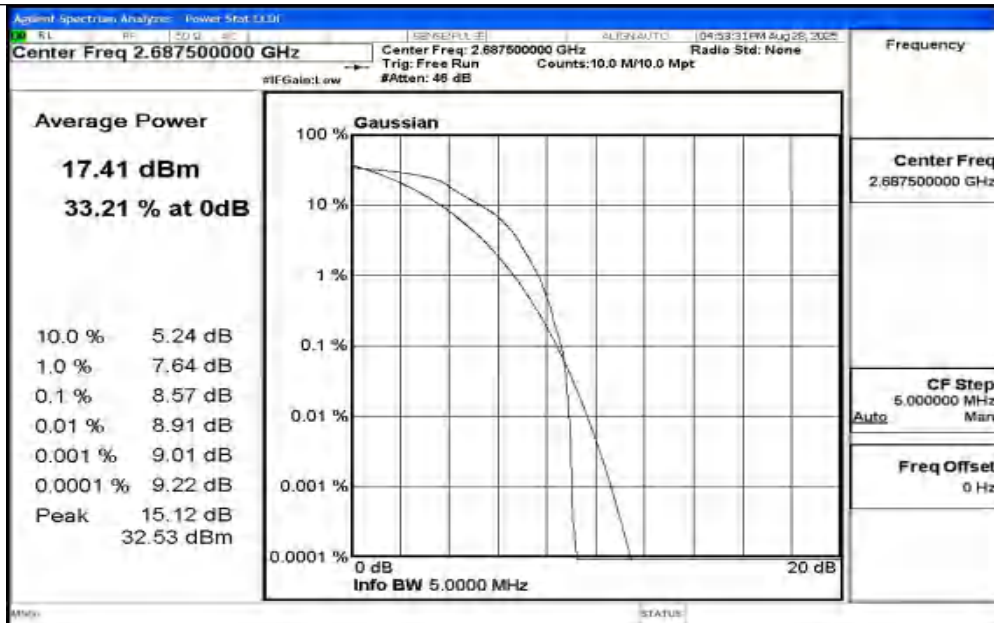
Band41-5MHz-QPSK-41565-1RB#0-PASS
