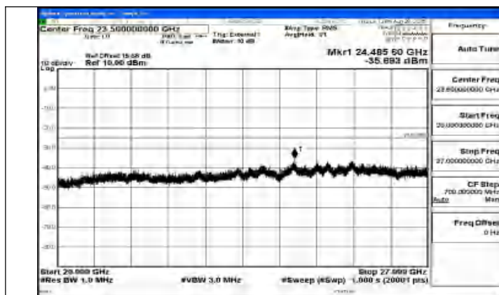
Band41_20MHz_QPSK_41490_1RB#0_20000~27000_20000~27000
