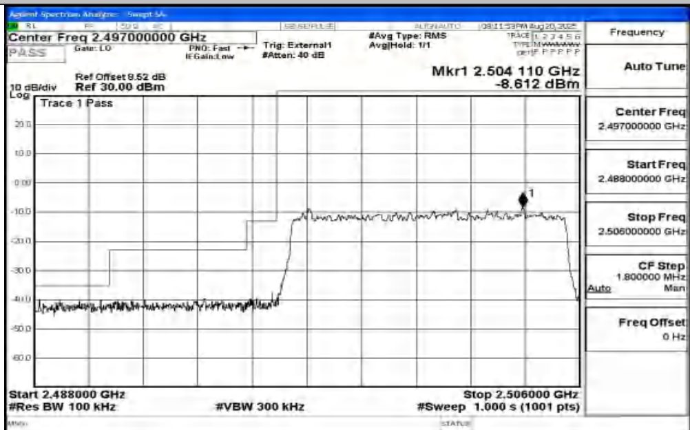
Band41_10MHz_16QAM_39700_50RB#0
