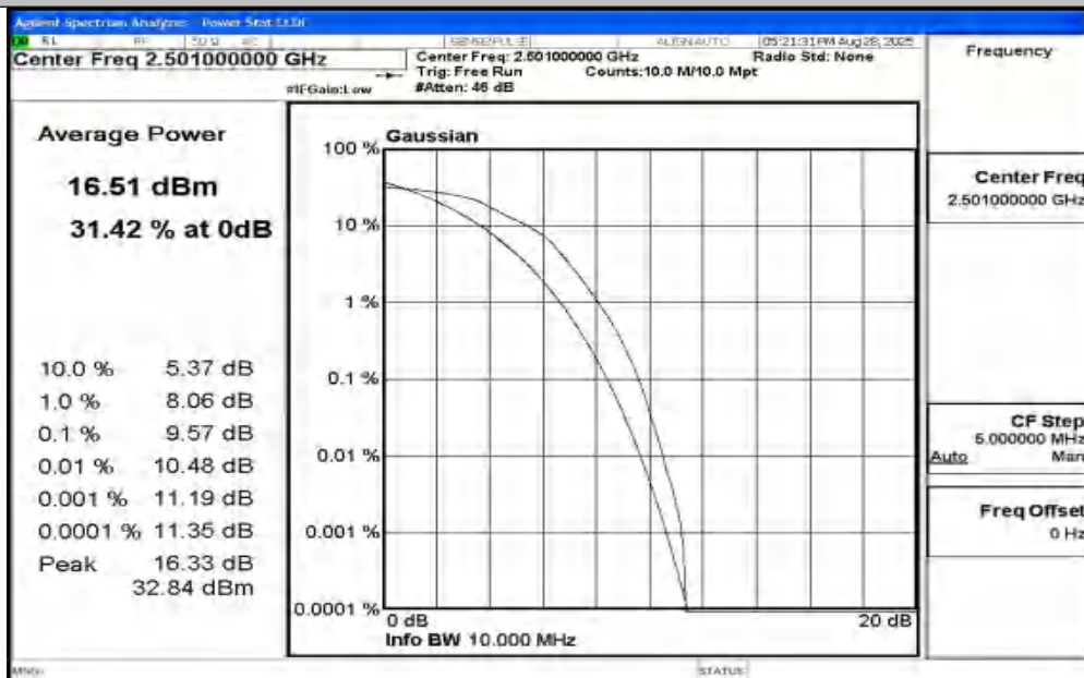
Band41-10MHz-16QAM-39700-50RB#0-PASS
