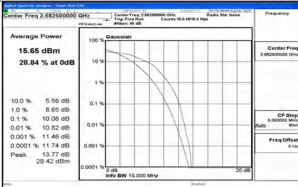
Band41-15MHz-16QAM-41515-75RB#0-PASS
