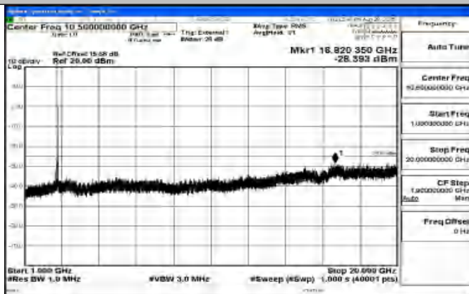
Band41_20MHz_16QAM_41490_1RB#0_1000~20000_1000~20000
