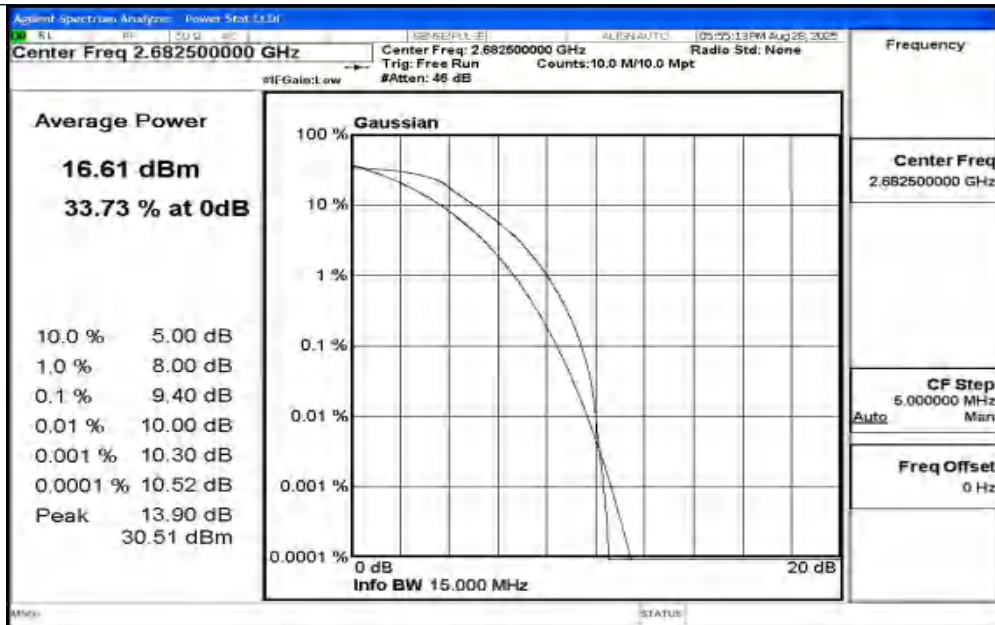
Band41-15MHz-QPSK-41515-75RB#0-PASS
