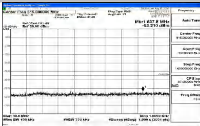
Band41_5MHz_QPSK_41565_1RB#0_30~1000_30~1000
