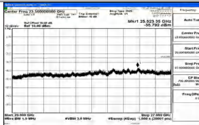
Band41_10MHz_16QAM_41540_1RB#0_20000~27000_20000~27000
