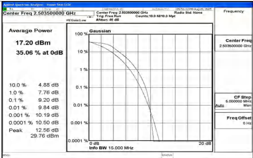
Band41-15MHz-QPSK-39725-75RB#0-PASS
