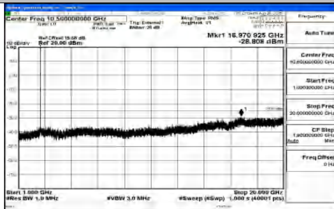
Band41_10MHz_16QAM_40620_1RB#0_1000~20000_1000~2000
