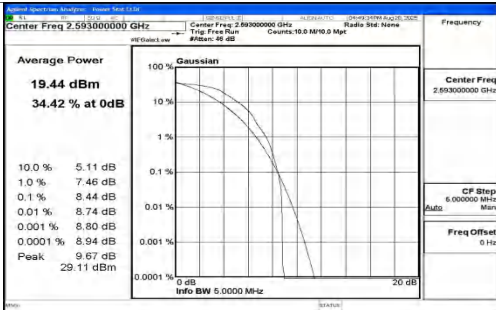
Band41-5MHz-QPSK-40620-1RB#0-PASS
