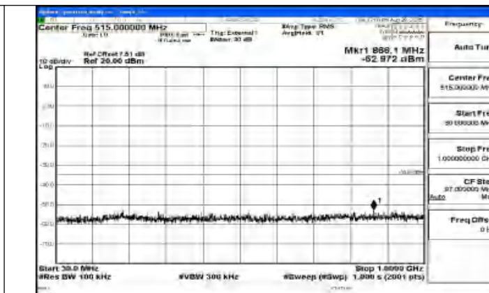
Band41_5MHz_16QAM_39675_1RB#0_30~1000_30~1000
