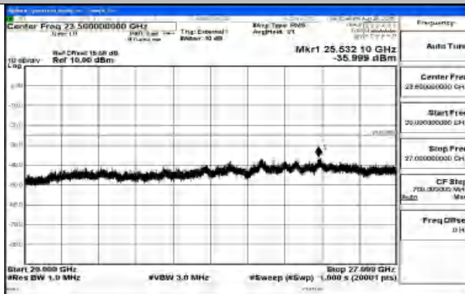
Band41_5MHz_QPSK_40620_1RB#0_20000~27000_20000~27000 0
