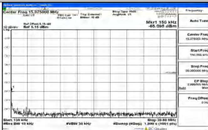
Band41_10MHz_16QAM_41540_1RB#0_0.15~30_0.15~30
