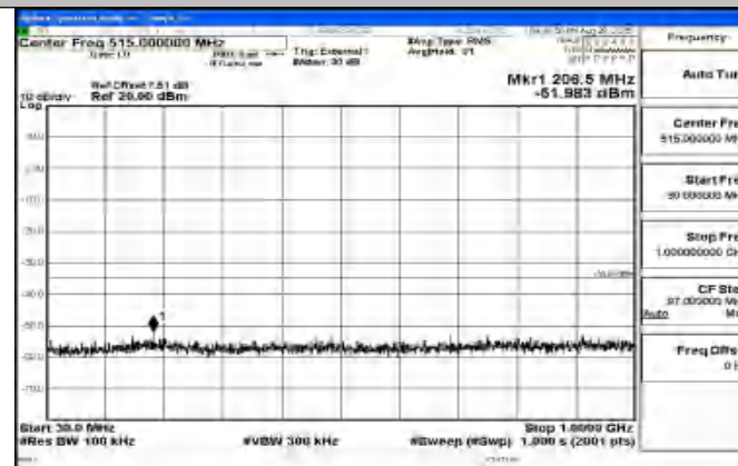
Band41_5MHz_16QAM_40620_1RB#0_30~1000_30~1000
