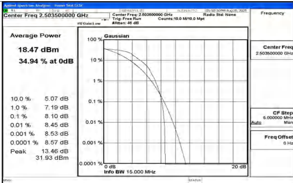
Band41-15MHz-QPSK-39725-1RB#0-PASS
