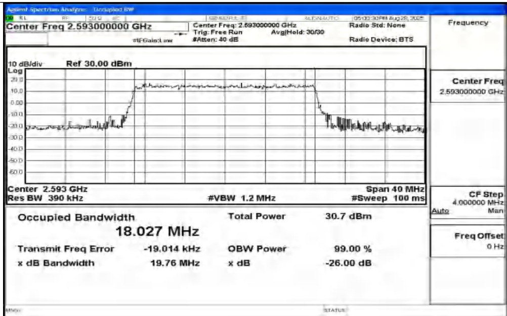
Band41-20MHz-QPSK-40620-100RB#0-PASS
