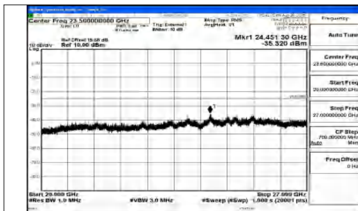
Band41_15MHz_QPSK_40620_1RB#0_20000~27000_20000~27000
