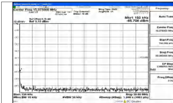
Band41_5MHz_16QAM_39675_1RB#0_0.15~30_0.15~30
