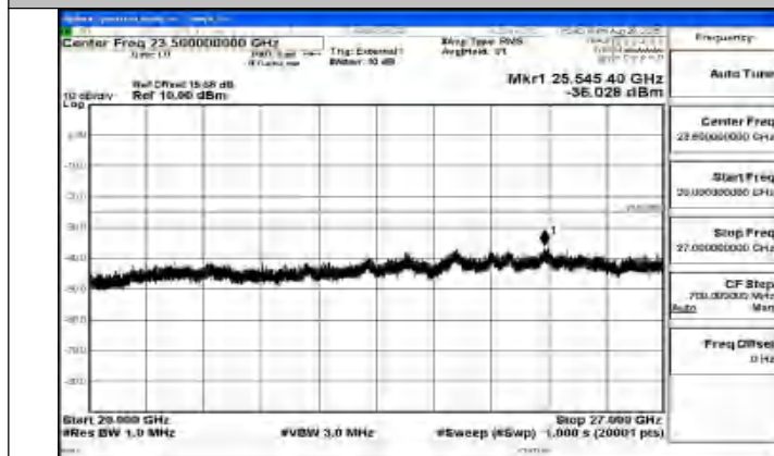
Band41_15MHz_QPSK_41515_1RB#0_20000~27000_20000~27000
