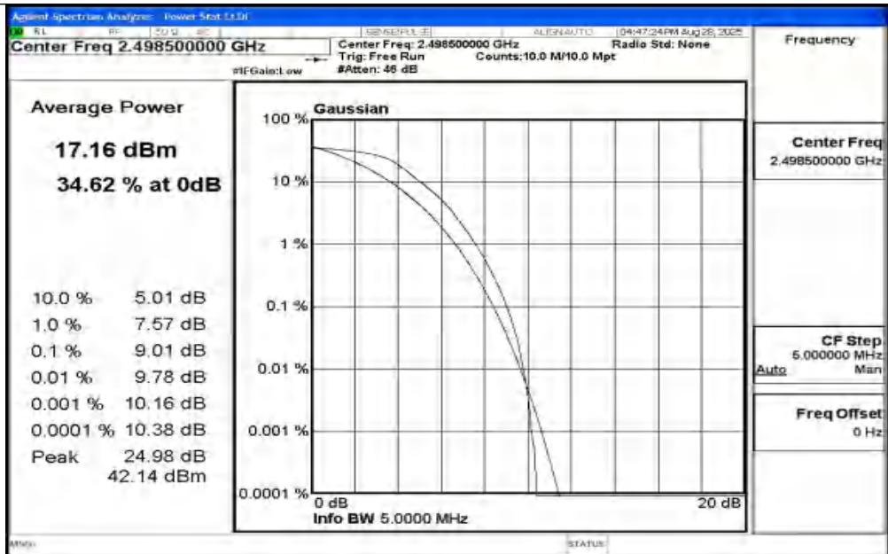
Band41-5MHz-QPSK-39675-25RB#0-PASS
