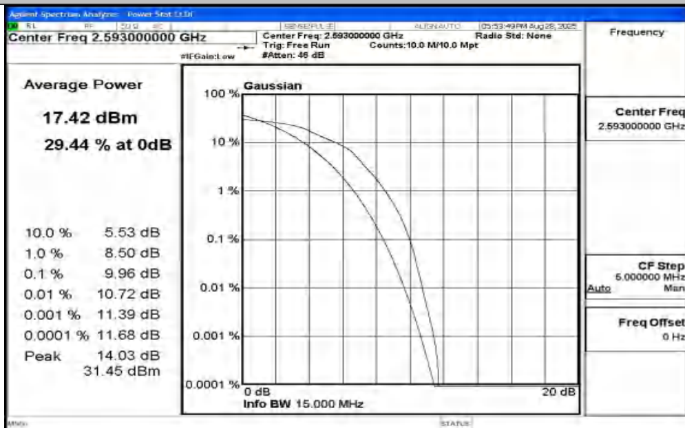
Band41-15MHz-16QAM-40620-75RB#0-PASS
