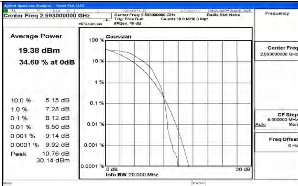
Band41-20MHz-QPSK-40620-1RB#0-PASS
