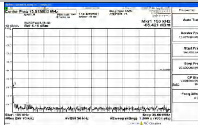
Band41_10MHz_QPSK_39700_1RB#0_0.15~30_0.15~30
