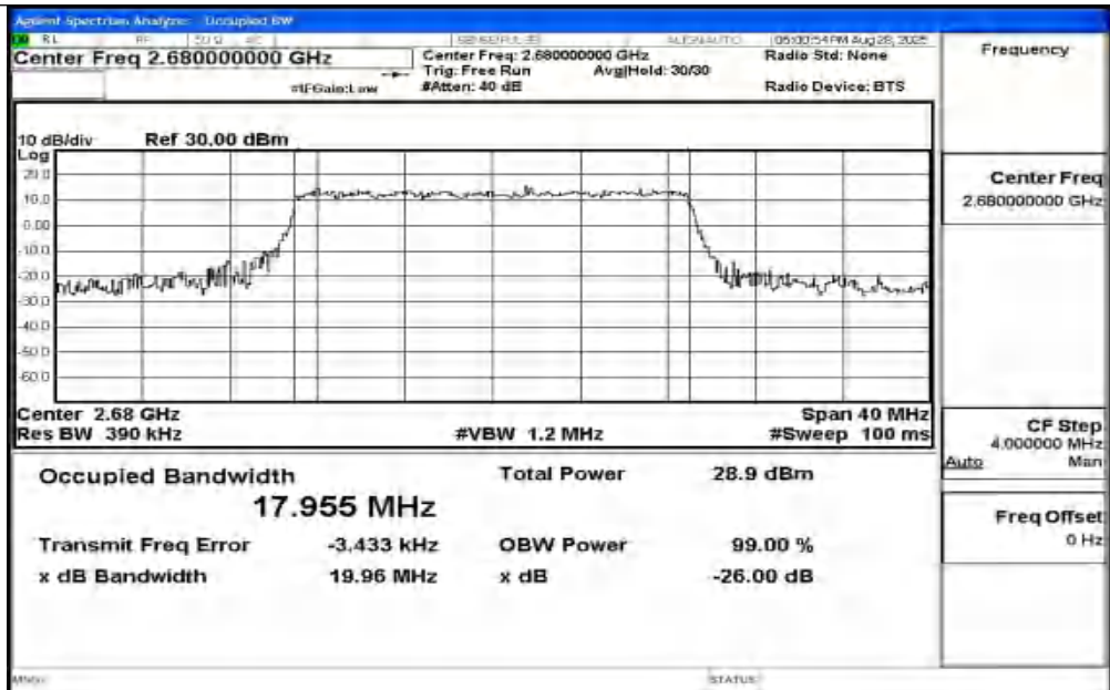
Band41-20MHz-QPSK-41490-100RB#0-PASS
