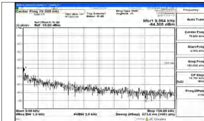
Band41_15MHz_QPSK_39725_1RB#0_0.009~0.15_0.009~0.15
