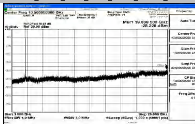
Band41_15MHz_QPSK_41515_1RB#0_1000~20000_1000~20000
