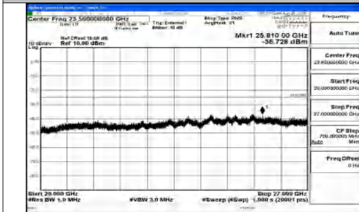
Band41_15MHz_QPSK_39725_1RB#0_20000~27000_20000~27000
