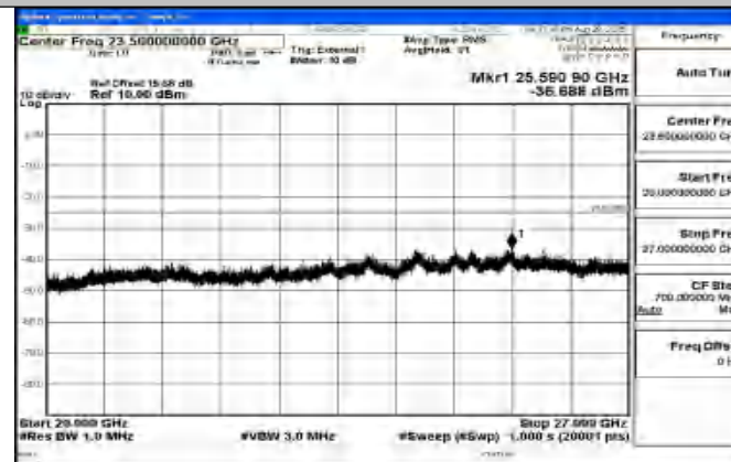
Band41_5MHz_16QAM_40620_1RB#0_20000~27000_20000~27000
