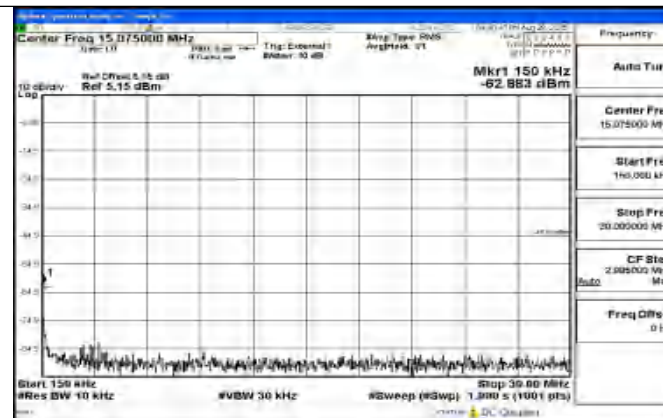
Band41_5MHz_QPSK_39675_1RB#0_0.15~30_0.15~30
