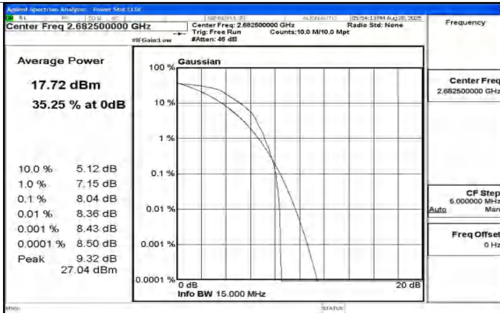
Band41-15MHz-QPSK-41515-1RB#0-PASS
