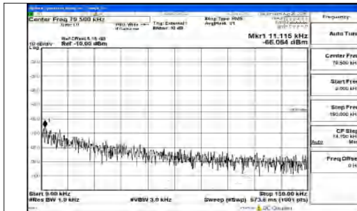
Band41_5MHz_QPSK_39675_1RB#0_0.009~0.15_0.009~0.15
