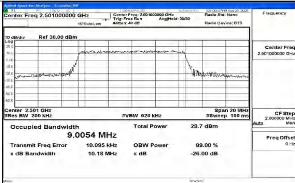
Band41-10MHz-16QAM-39700-50RB#0-PASS
