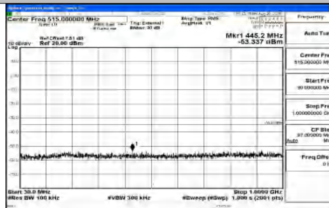
Band41_10MHz_16QAM_41540_1RB#0_30~1000_30~1000
