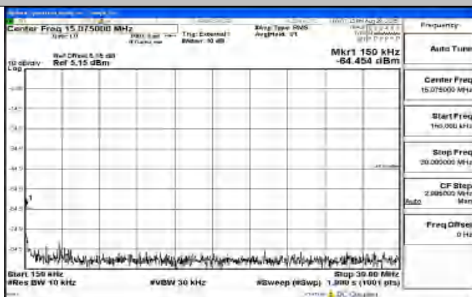
Band41_20MHz_16QAM_39750_1RB#0_0.15~30_0.15~30
