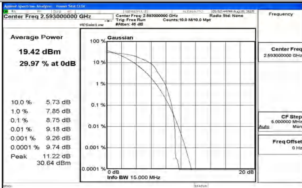
Band41-15MHz-16QAM-40620-1RB#0-PASS
