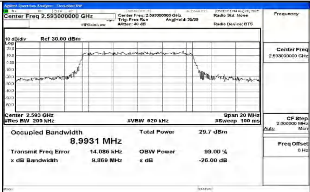
Band41-10MHz-16QAM-40620-50RB#0-PASS
