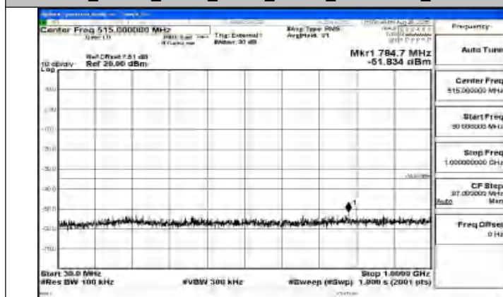
Band41_10MHz_QPSK_40620_1RB#0_30~1000_30~1000
