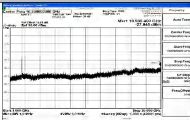
Band41_20MHz_16QAM_39750_1RB#0_1000~20000_1000~20000
