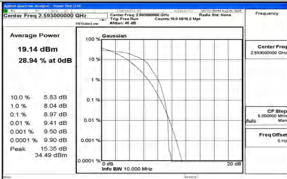
Band41-10MHz-16QAM-40620-1RB#0-PASS
