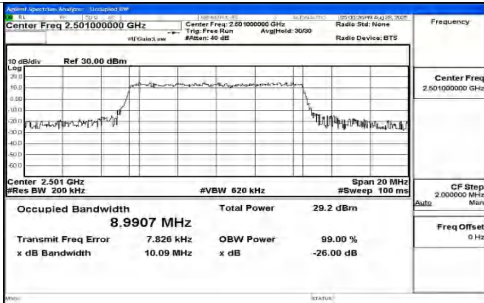
Band41-10MHz-QPSK-39700-50RB#0-PASS
