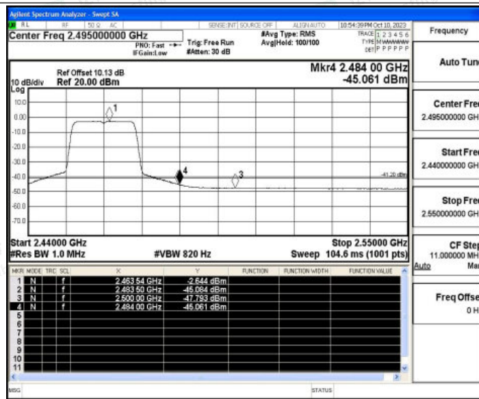
11N20SISO_Ant1_High_2462_Peak
