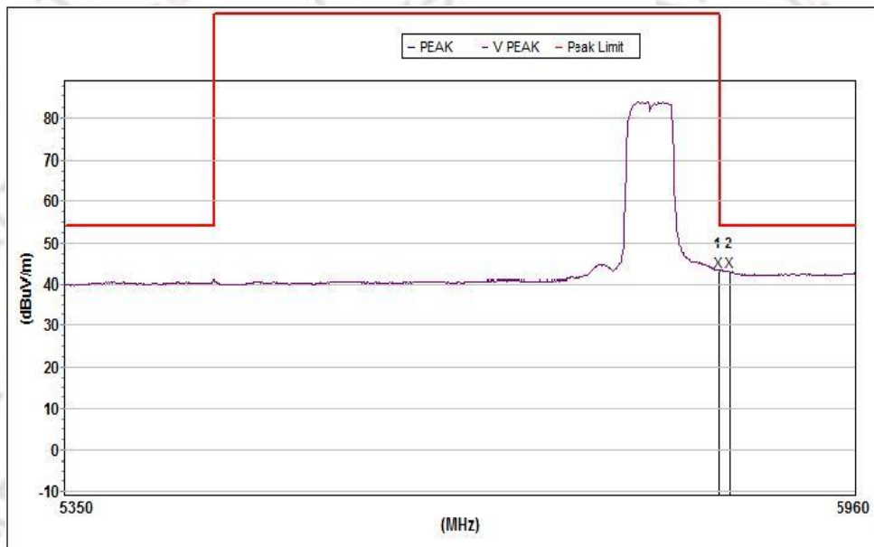
5795MHz Vertical
