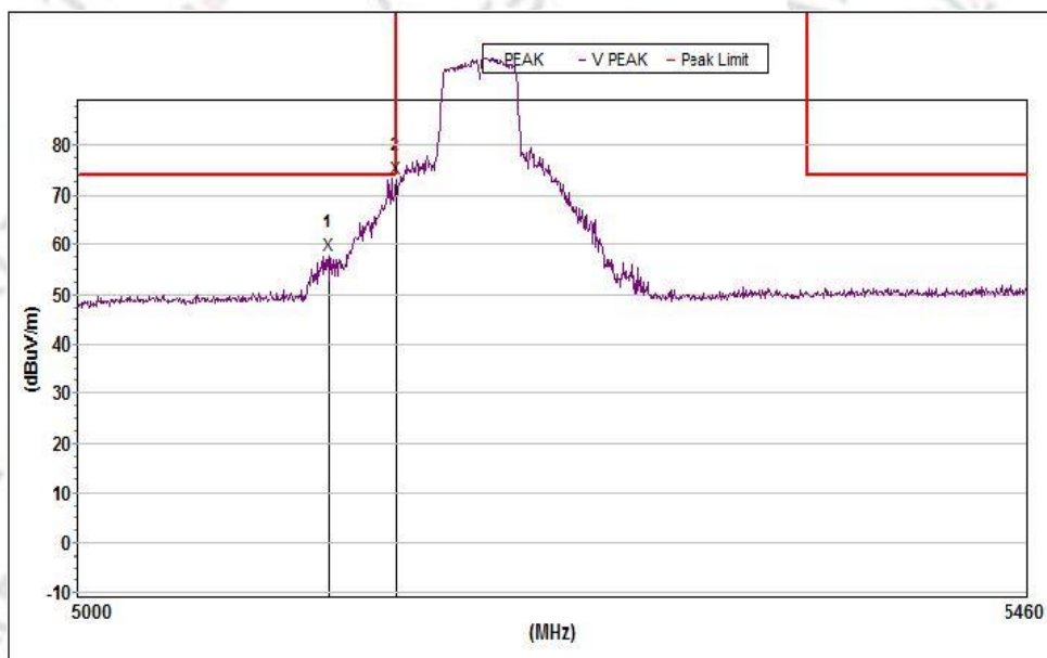
5190MHz Vertical
