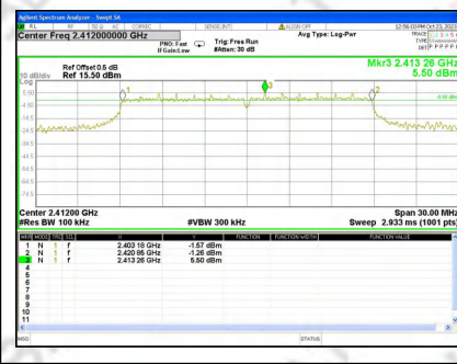
6dB Bandwidth Mode7 CH 01
