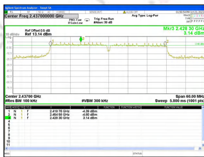
6dB Bandwidth Mode11 CH 06
