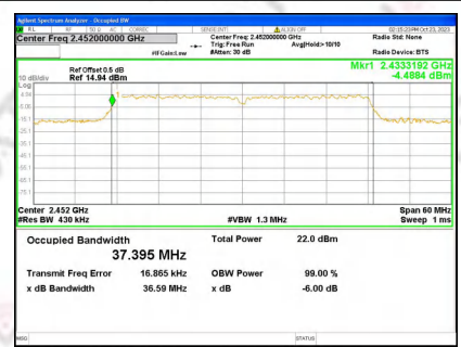
99% Bandwidth Mode12 CH 09
