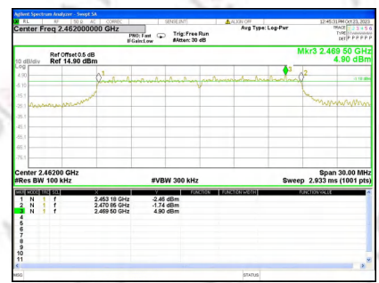
6dB Bandwidth Mode9 CH 11
