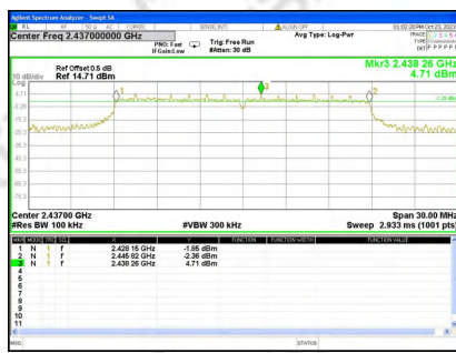
6dB Bandwidth Mode8 CH 06
