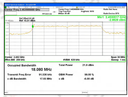
99% Bandwidth Mode9 CH 11
