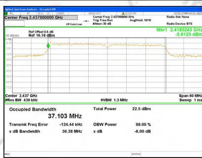
99% Bandwidth Mode11 CH 06
