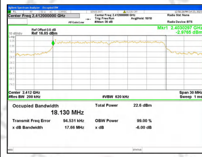
99% Bandwidth Mode7 CH 01
