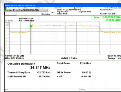
99% Bandwidth Mode10 CH 03
