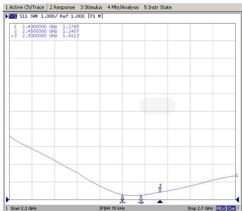
SWR
