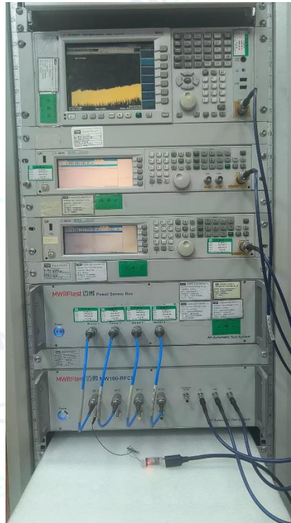
Photo of Setup for RF Conducted
