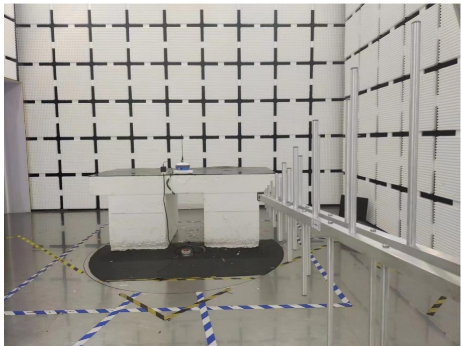
Radiation Emission View(Below 1GHz)
