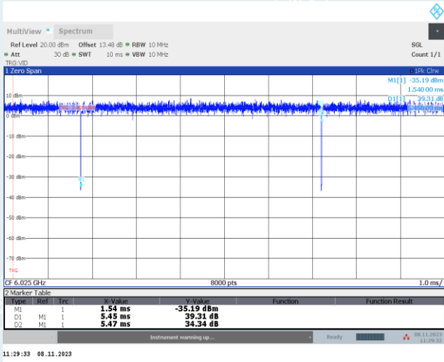
IEEE 802.11ax HE160_Ant2_6025MHz
