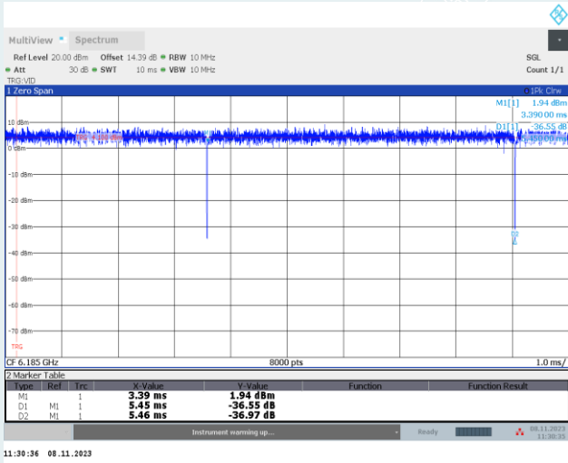
IEEE 802.11ax HE160_Ant2_6185MHz
