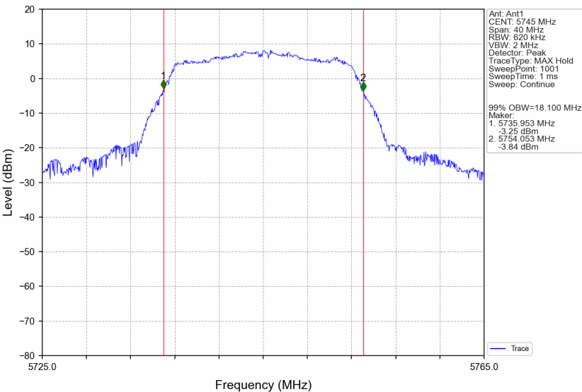
802.11a_LCH_5745MHz_Ant1_NTNV
