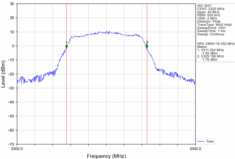
802.11a_HCH_5320MHz_Ant1_NTNV
