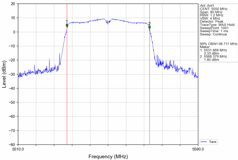
802.11ac(VHT40)_MCH_5550MHz_Ant1_NTNV
