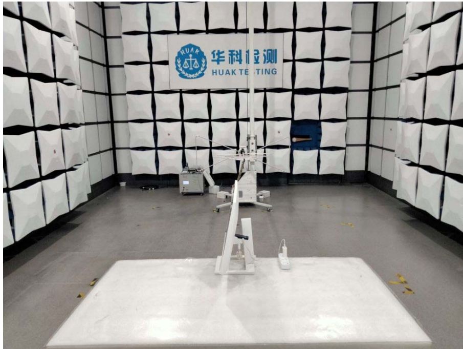
Model: Lite 2 Rx Radiated Emissions
