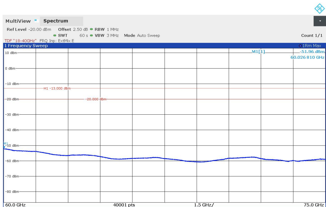
Plots No. 27: Spurious Emission at Antenna Terminal, RMS detector / 16QAM Modulation / 60 GHz – 75 GHz
