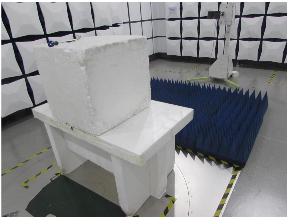
BT/FM Radiated Emission Above 1GHz
