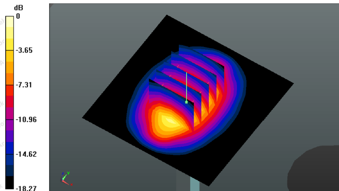
System Performance Check 1900MHz Head 250mW
