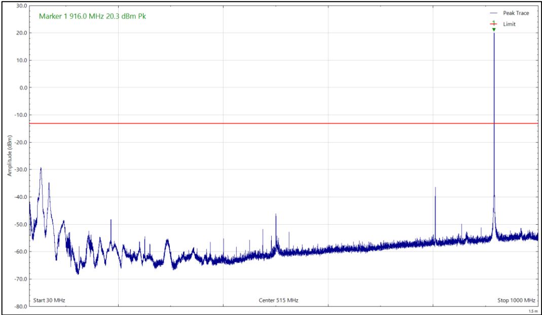
Figure 8 – 30 MHz to 1 GHz, Peak, Vertical
