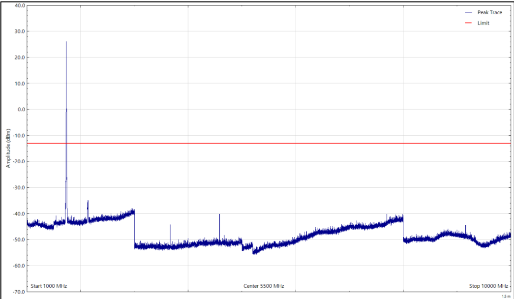
Figure 7 - 1 GHz to 10 GHz, Peak, Horizontal
