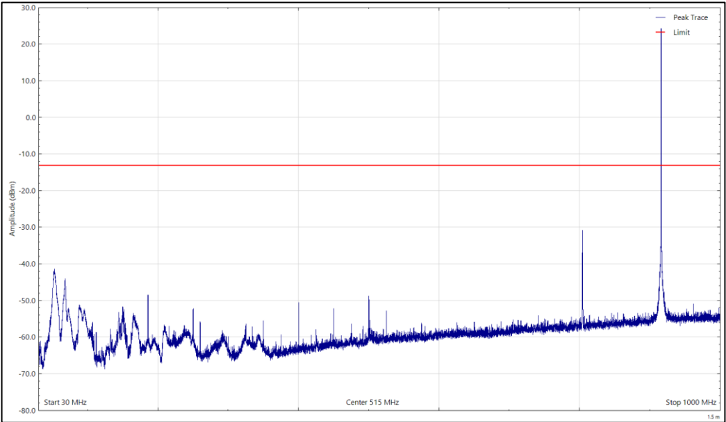
Figure 6 - 30 MHz to 1 GHz, Peak, Horizontal
