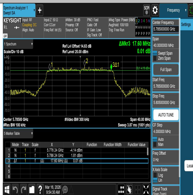
11AX20SISO-Ant1-5785-PASS
