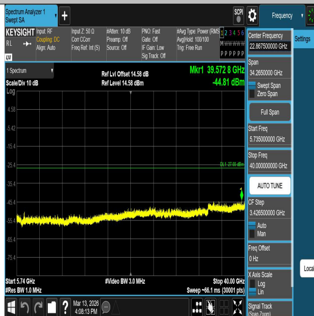
11AC20SISO-Ant1-5580-5735~40000-PASS
