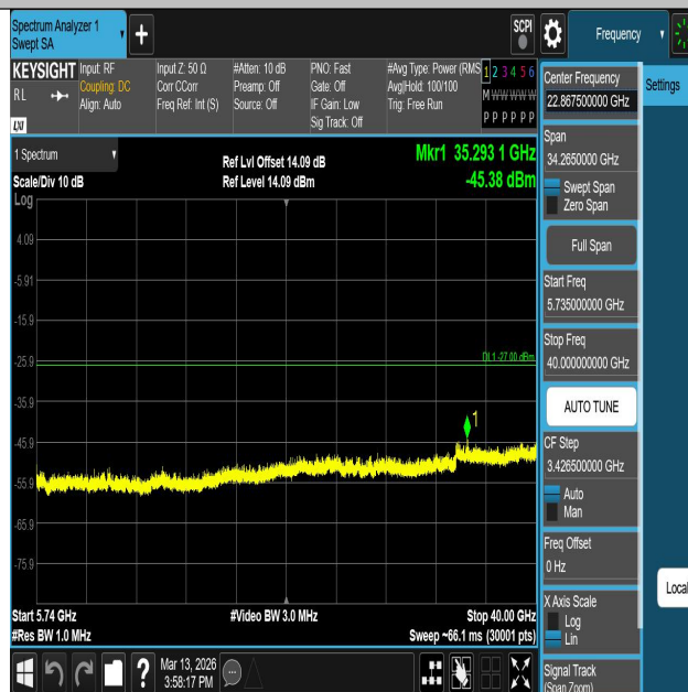
11AC20SISO-Ant1-5500-5735~40000-PASS
