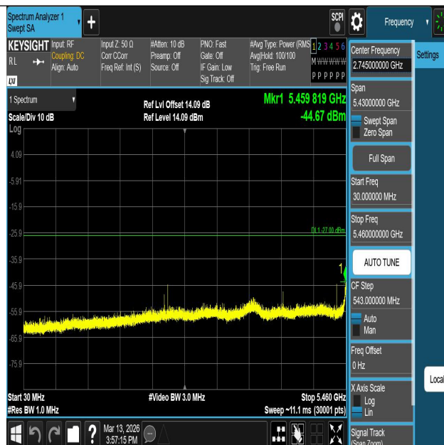
11AC20SISO-Ant1-5500-30~5460-PASS
