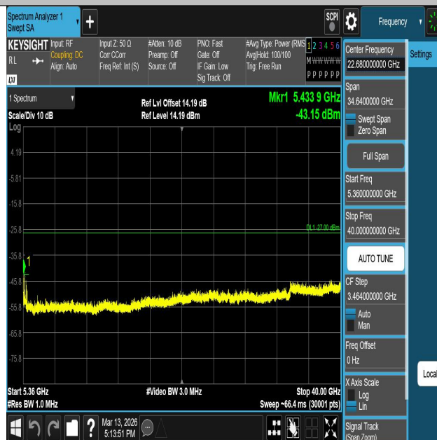
11AC40SISO-Ant1-5310-5360~40000-PASS
