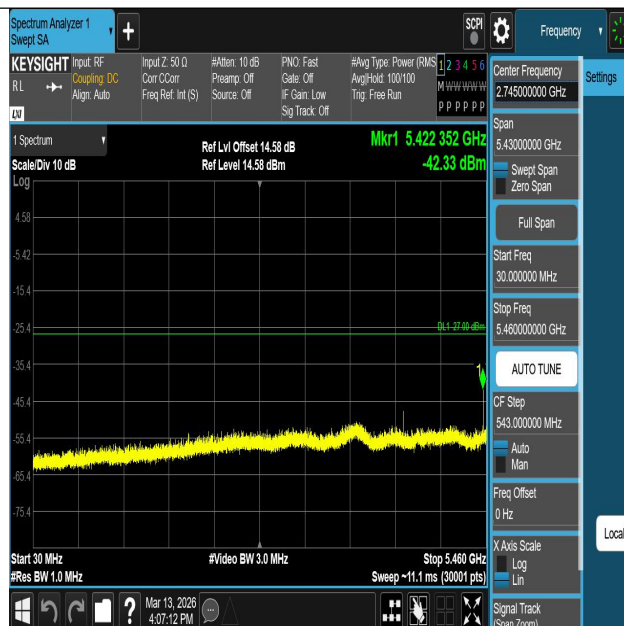
11AC20SISO-Ant1-5580-30~5460-PASS
