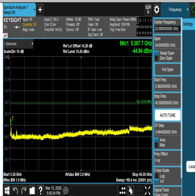
11AC40SISO-Ant1-5270-5360~40000-PASS
