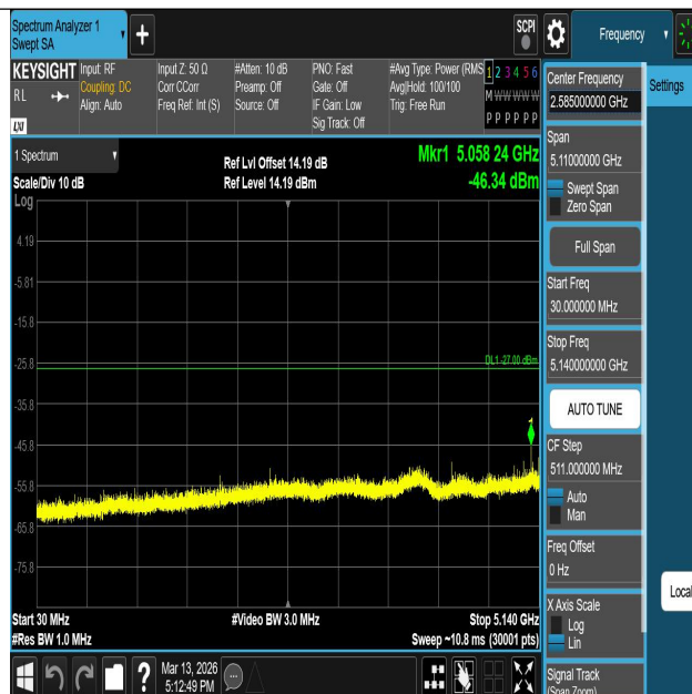
11AC40SISO-Ant1-5310-30~5140-PASS
