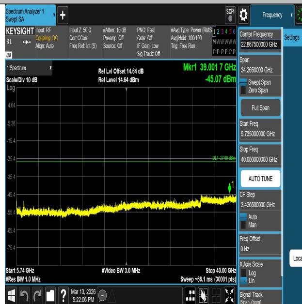
11AC40SISO-Ant1-5510-5735~40000-PASS
