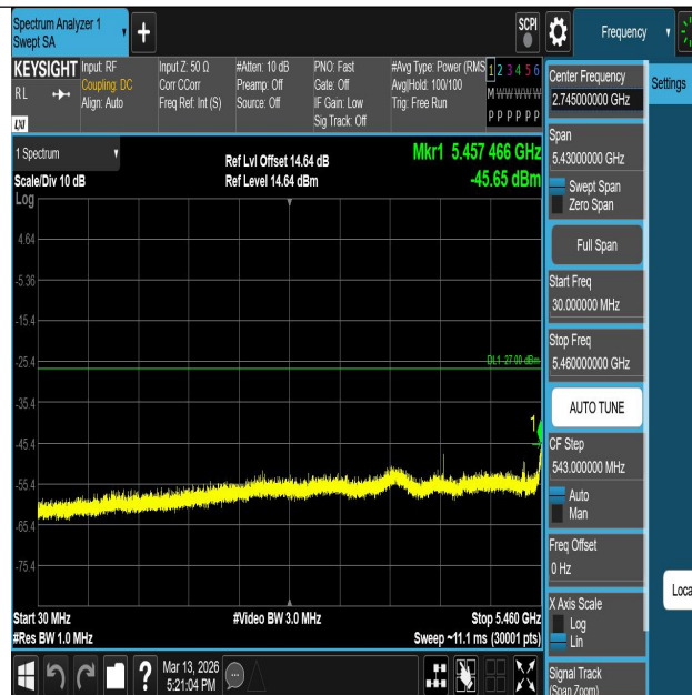
11AC40SISO-Ant1-5510-30~5460-PASS
