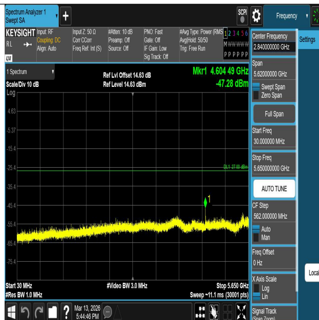
11AC40SISO-Ant1-5755-30~5650-PASS
