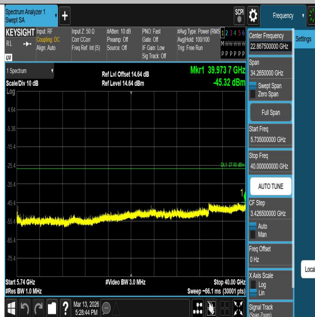
11AC40SISO-Ant1-5550-5735~40000-PASS
