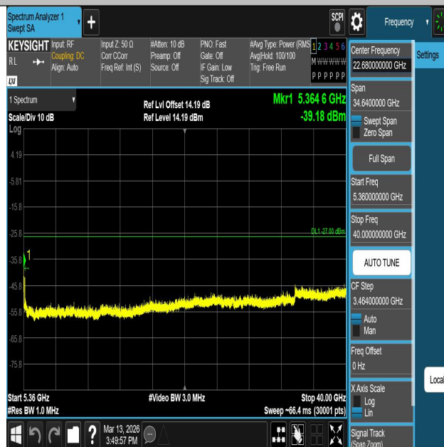
11AC20SISO-Ant1-5320-5360~40000-PASS
