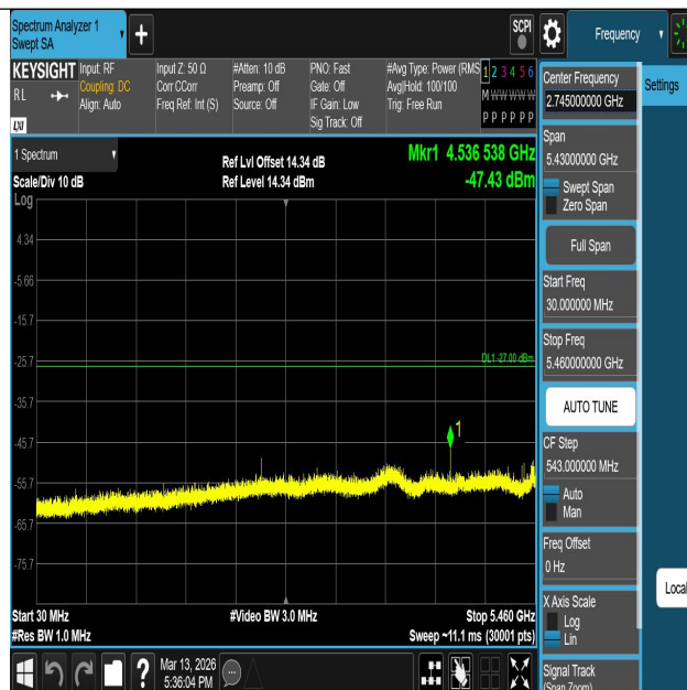
11AC40SISO-Ant1-5670-30~5460-PASS
