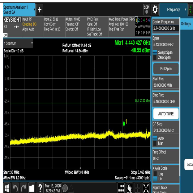
11AC40SISO-Ant1-5550-30~5460-PASS
