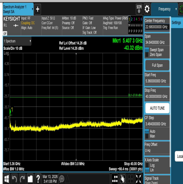
11AC20SISO-Ant1-5280-5360~40000-PASS
