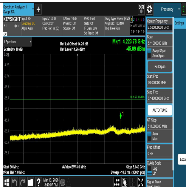
11AC20SISO-Ant1-5280-30~5140-PASS
