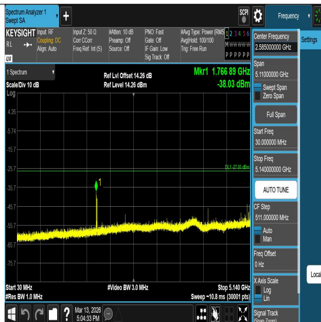
11AC40SISO-Ant1-5270-30~5140-PASS
