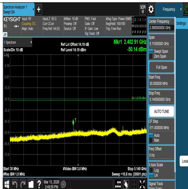
11AC20SISO-Ant1-5320-30~5140-PASS
