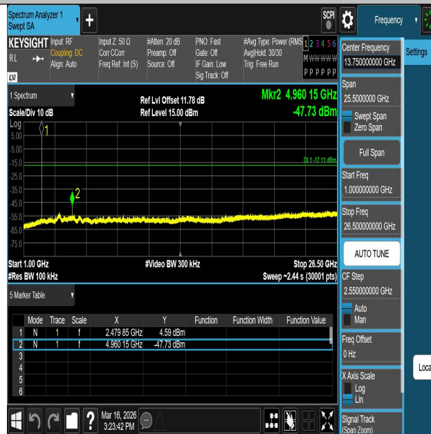
2DH5-Ant1-2480-1000~26500-PASS
