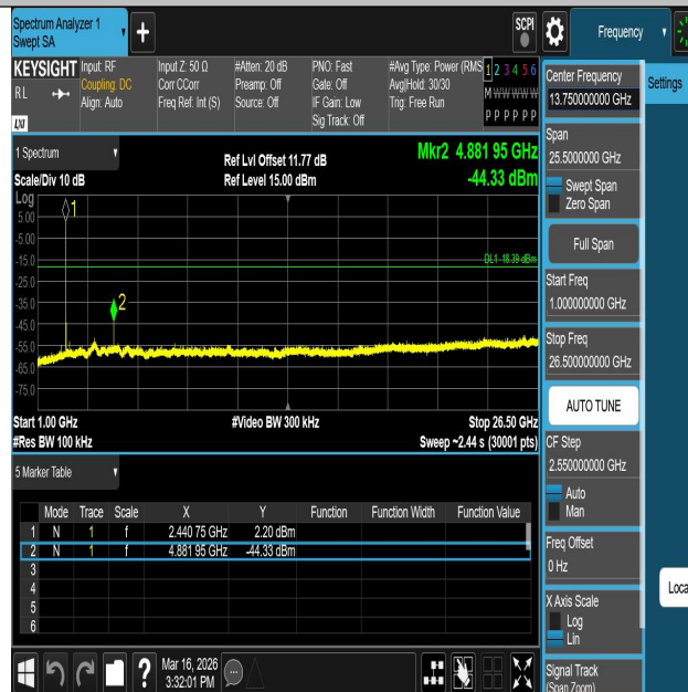
3DH5-Ant1-2441-1000~26500-PASS
