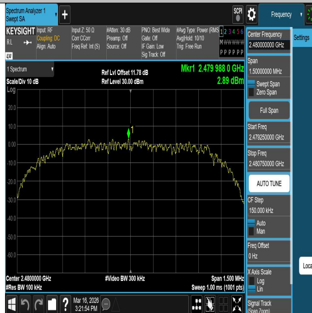
2DH5-Ant1-2480-0~Reference-PASS
