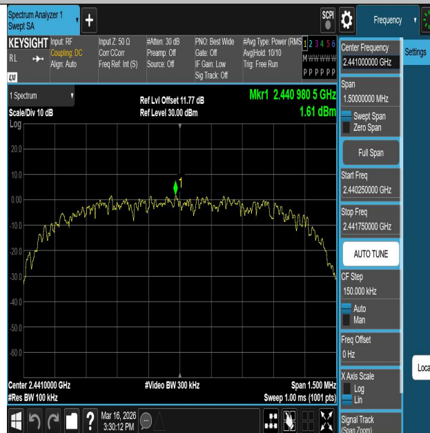
3DH5-Ant1-2441-0~Reference-PASS
