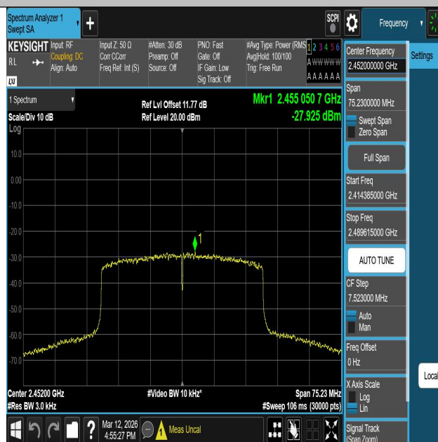
11AX40SISO-Ant1-2452-PASS
