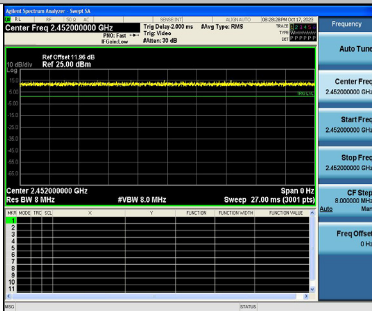
NTNV-11N40SISO-Ant1-2452
