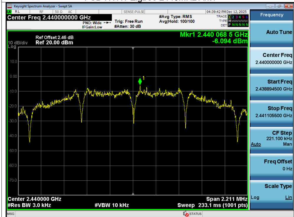
PSD NVNT Zigbee 2440MHz Ant1
