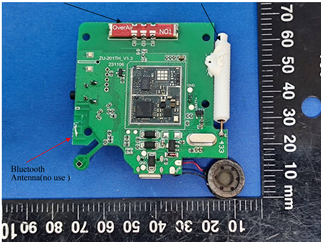
433.92MHz Rx Antenna
