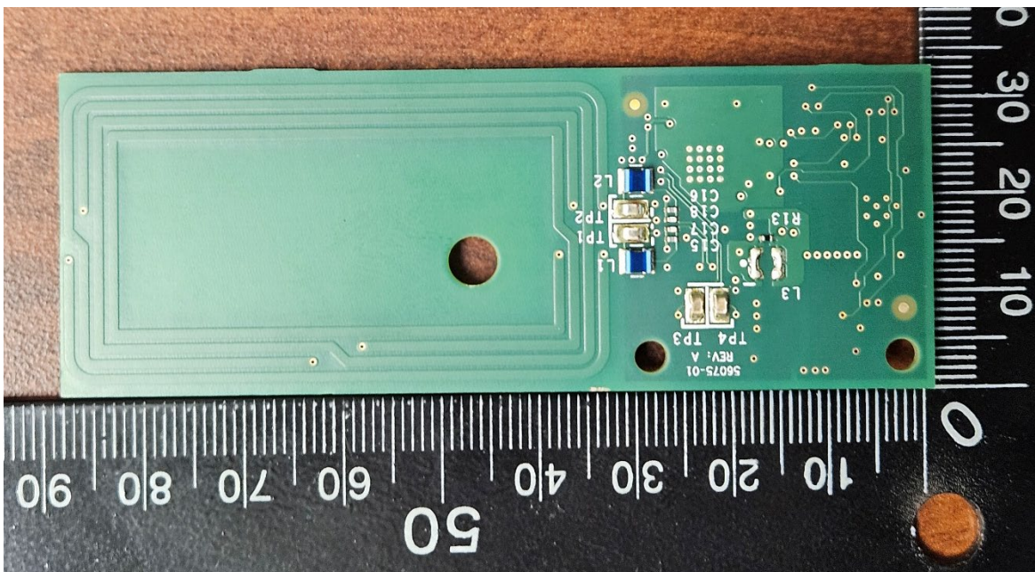
NFC radio with trace antenna
