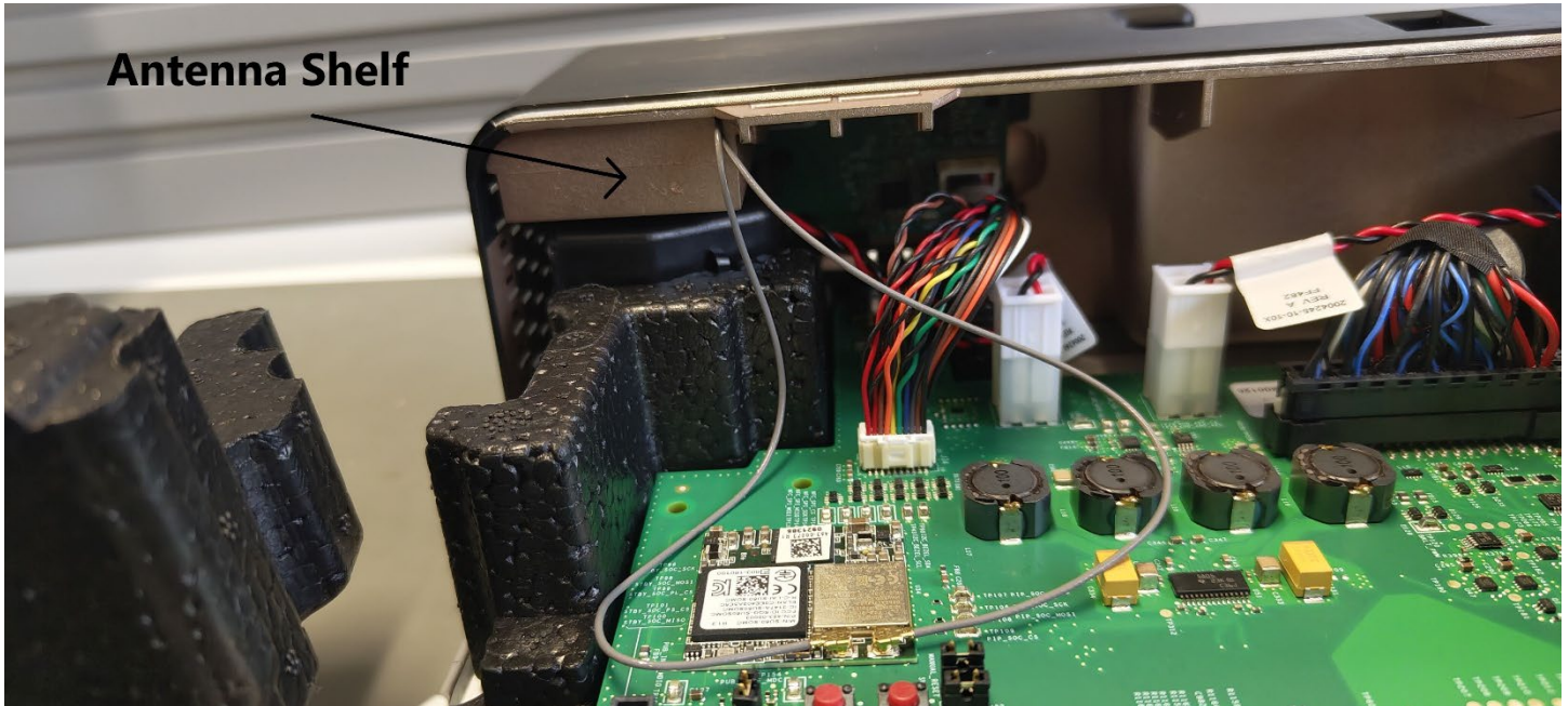
WiFi Module with antenna
