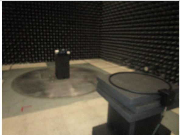
Skew Loop Antenna
