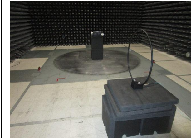
Perpendicular Loop Antenna
