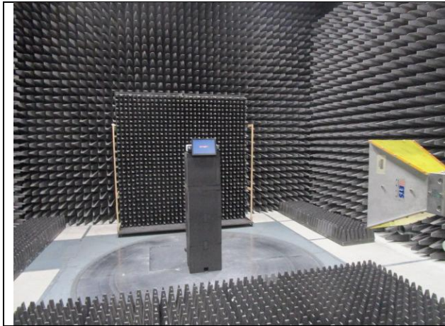
Spurious / Simultaneous transmit 1-18 GHz
