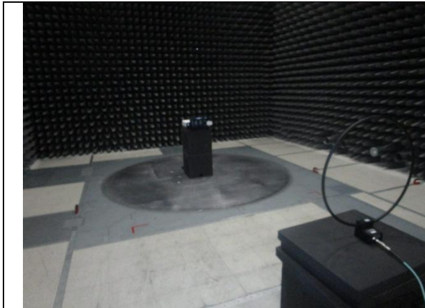
Parallel Loop Antenna
