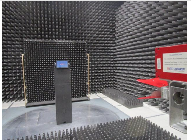
Spurious / Simultaneous transmit 18-40 GHz
