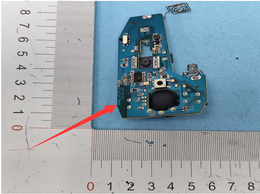
Antenna Photo & Length (mm)
