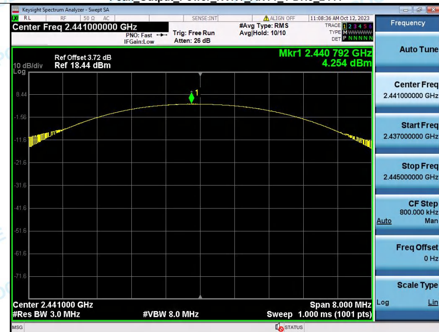
Peak Output Power_NVNT_ANT1_1-DH5_2441
