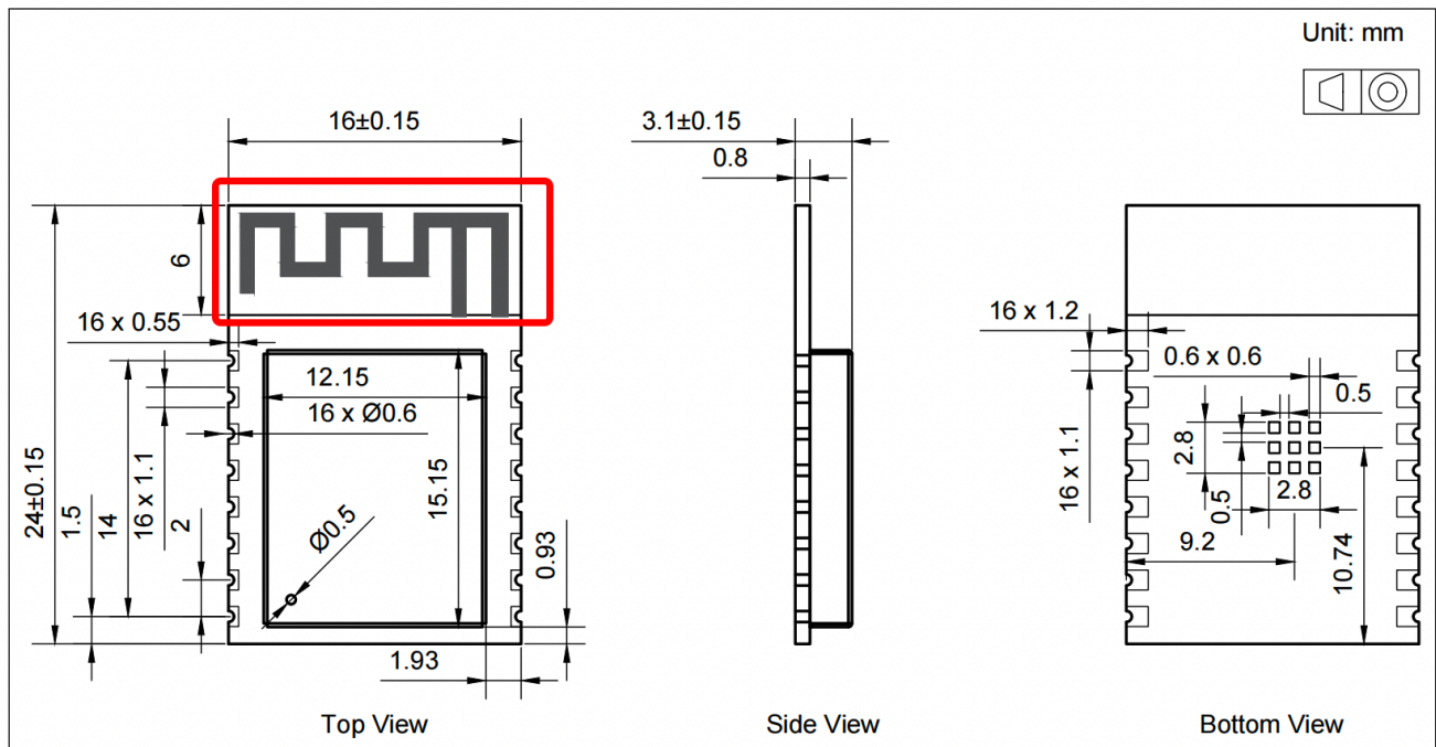
Picture 1 Antenna plots
