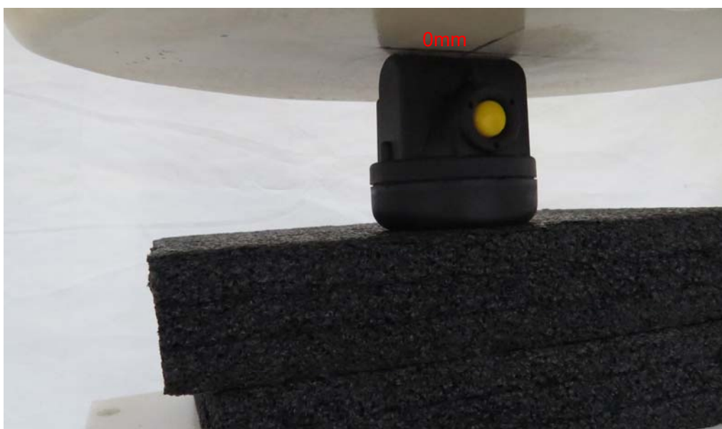
Picture 6: Bottom Edge, the distance from EUT to the bottom of the Phantom is 0mm
