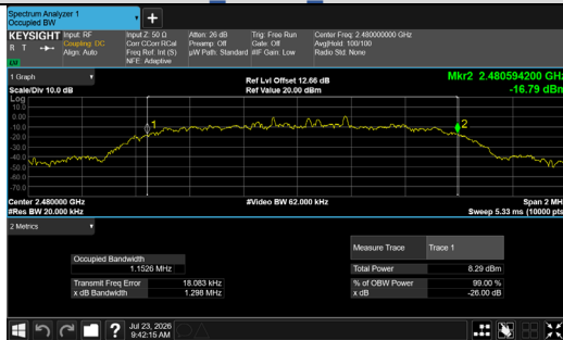
8DPSK 3-DH5 Channel 78
