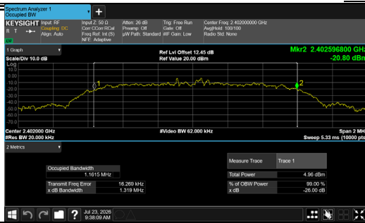
8DPSK 3-DH5 Channel 0
