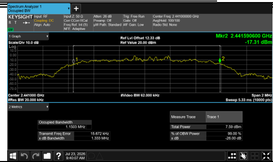
8DPSK 3-DH5 Channel 39
