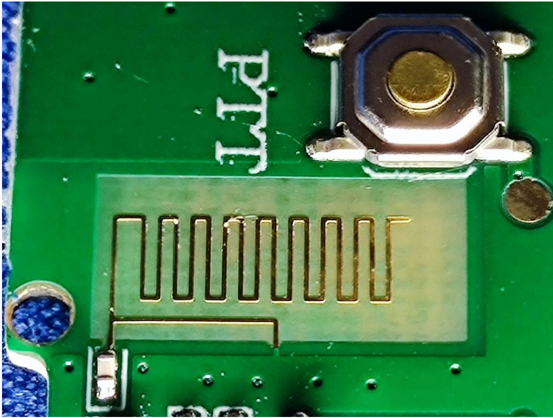
receiving antenna
