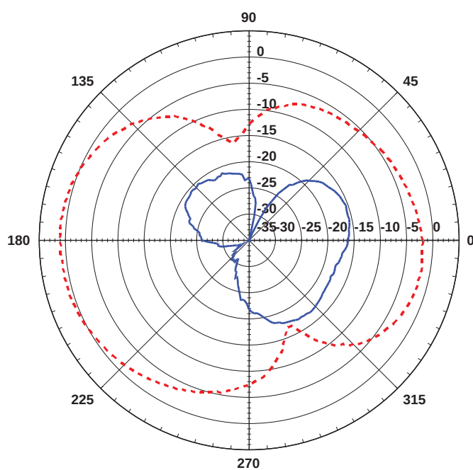
Co-cross polarization field (dBi)
