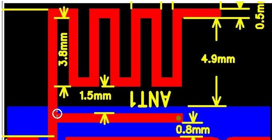
3-1 Normal Module Wigggle Antenna
