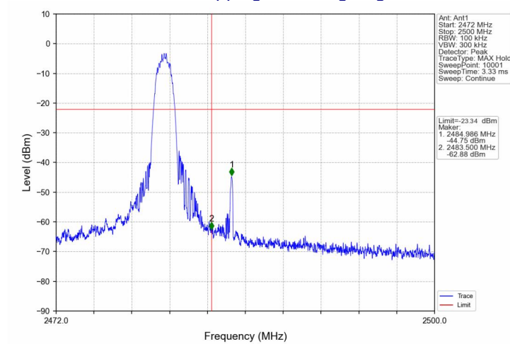
8-DPSK No-hopping Band edge-right side
