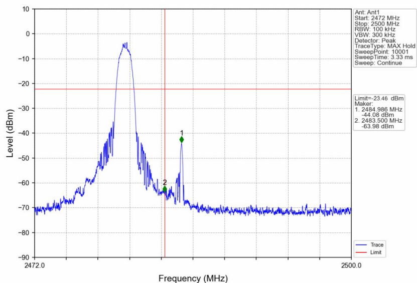
\pi/4 -DQPSK Hopping Band edge-right side
