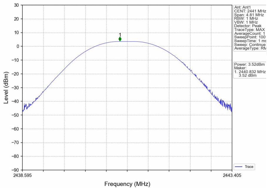
GFSK Middle Channel
