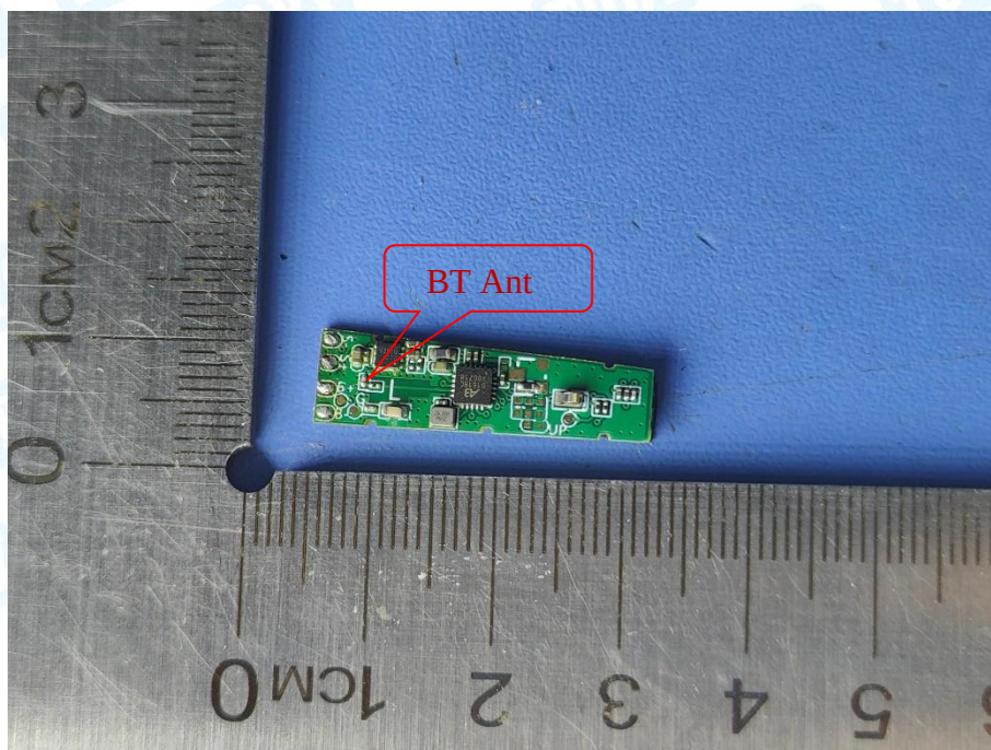
Photo 10 Appearance of PCB (Right)
