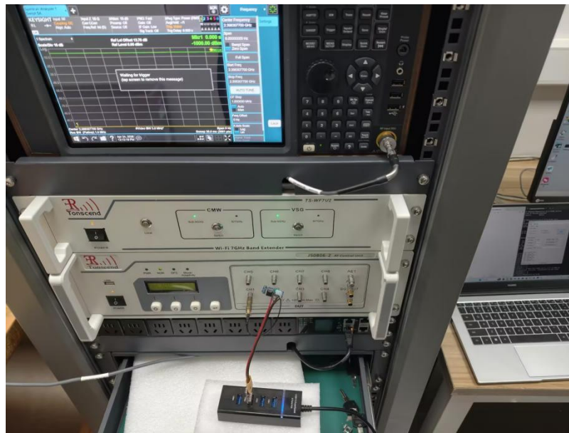
RF conducted-Left side
