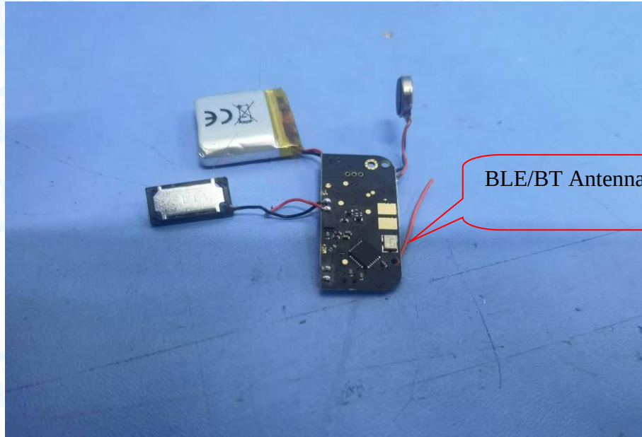
Photo 14 Appearance of PCB & Battery
