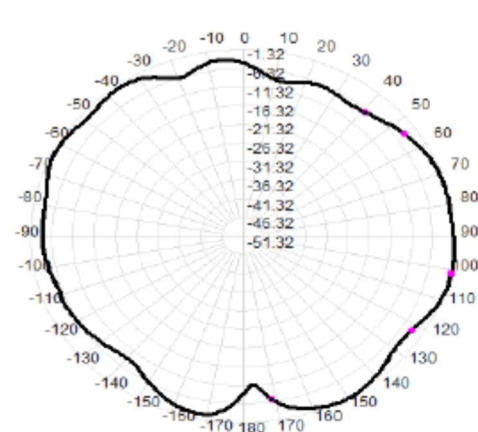
Fig. 5 E2 surface - total gain direction plot
