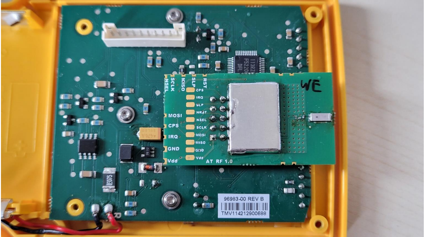
Photo No. 9: radiated sample (installed in test jig)
