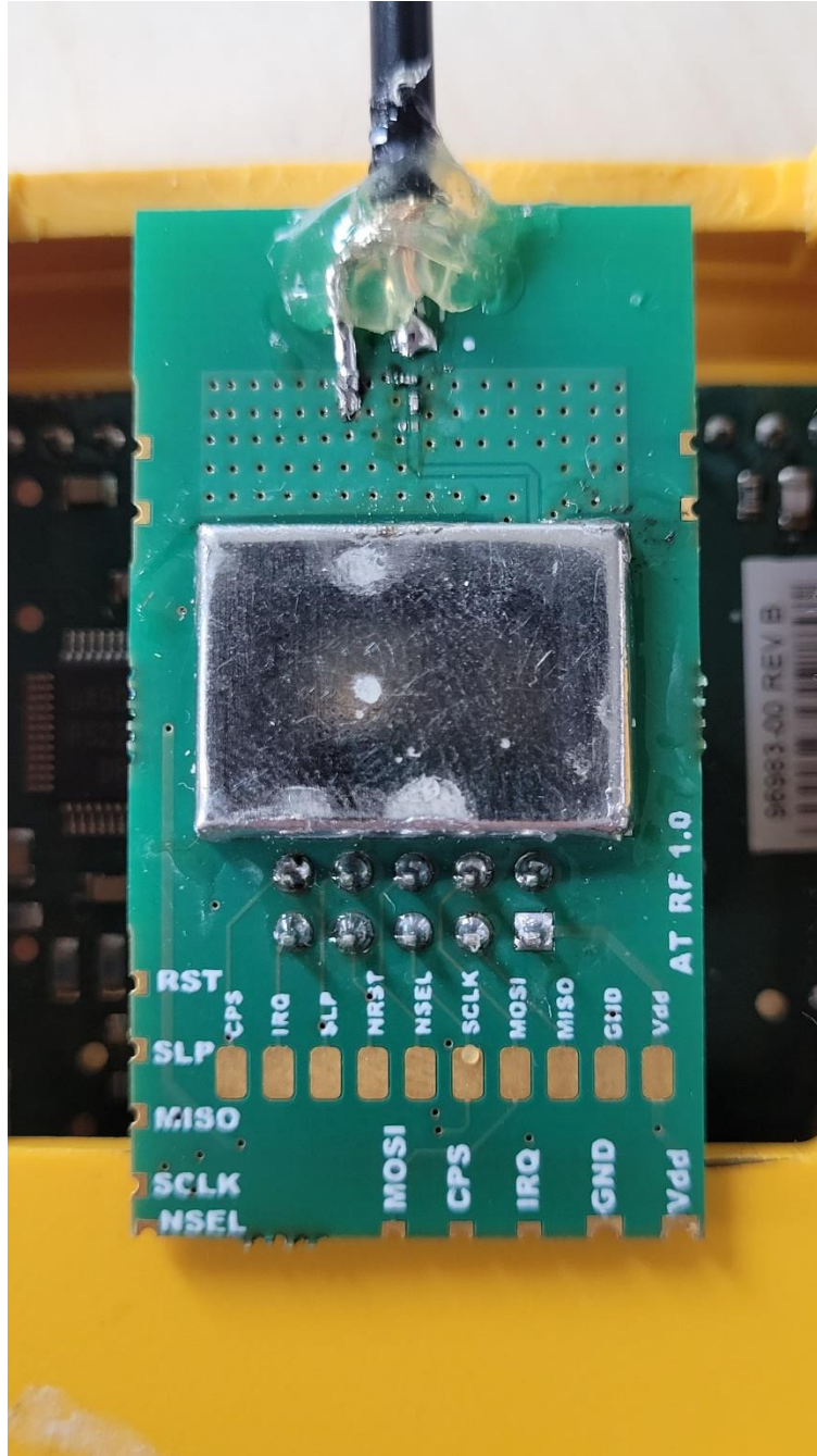
Photo No. 7: conducted sample (module installed in test jig)
