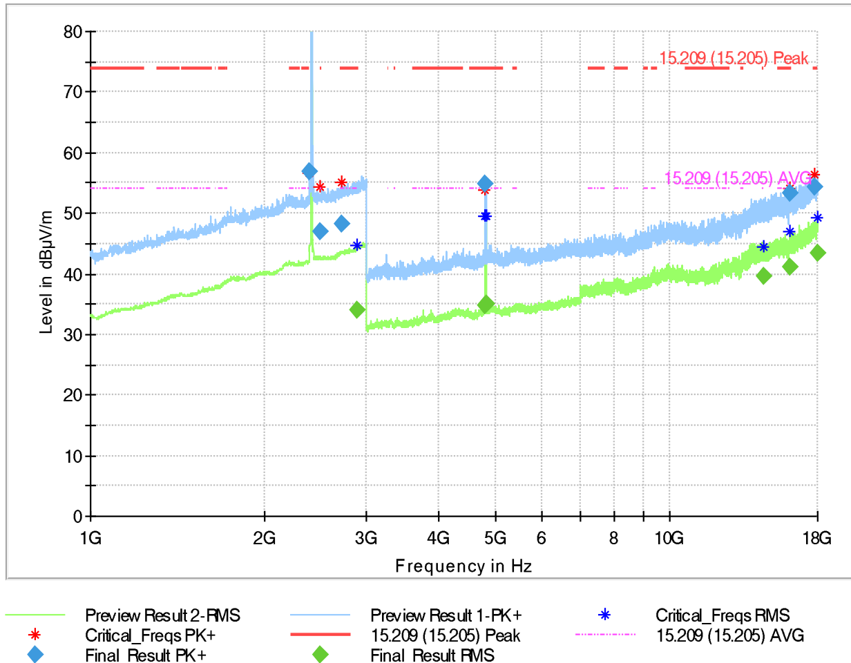
Plot 24: Mode 1, RSE 1 GHz – 18 GHz, low channel, horizontal / vertical polarisation
