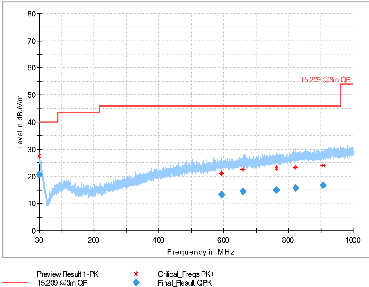
Plot 22: Mode 1, RSE 30 MHz – 1 GHz, low channel, horizontal / vertical polarisation
