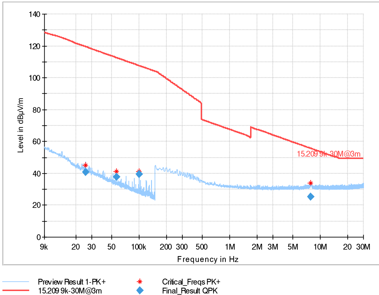
Plot 21: Mode 1, RSE 9 kHz – 30 MHz, high channel, loop antenna
