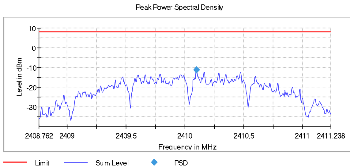
Plot 10: Mode 1, Peak PSD, low channel
