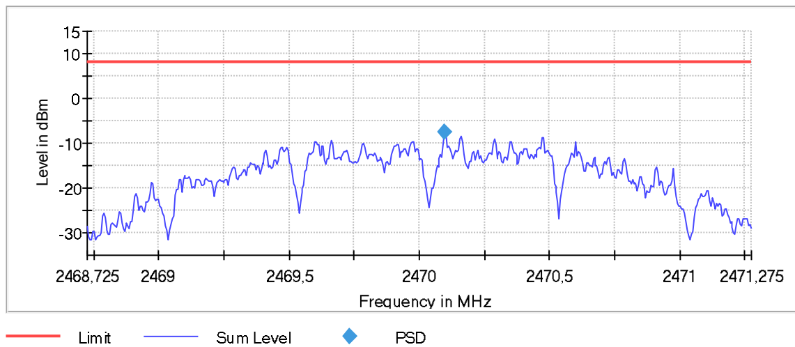
Plot 12: Mode 1, Peak PSD, high channel
