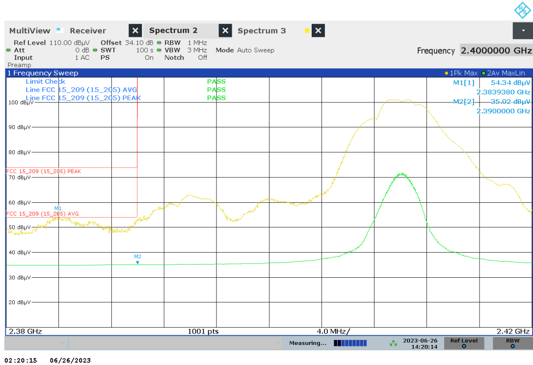
Plot 15: Mode 1, BEC, low channel
