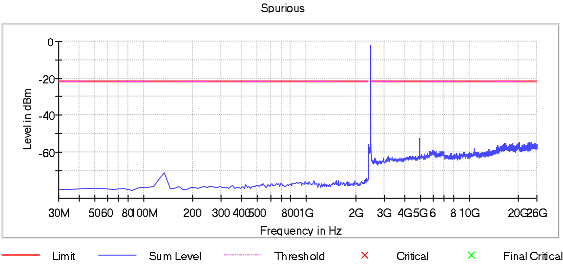
Plot 19: Mode 1, CSE, high channel
