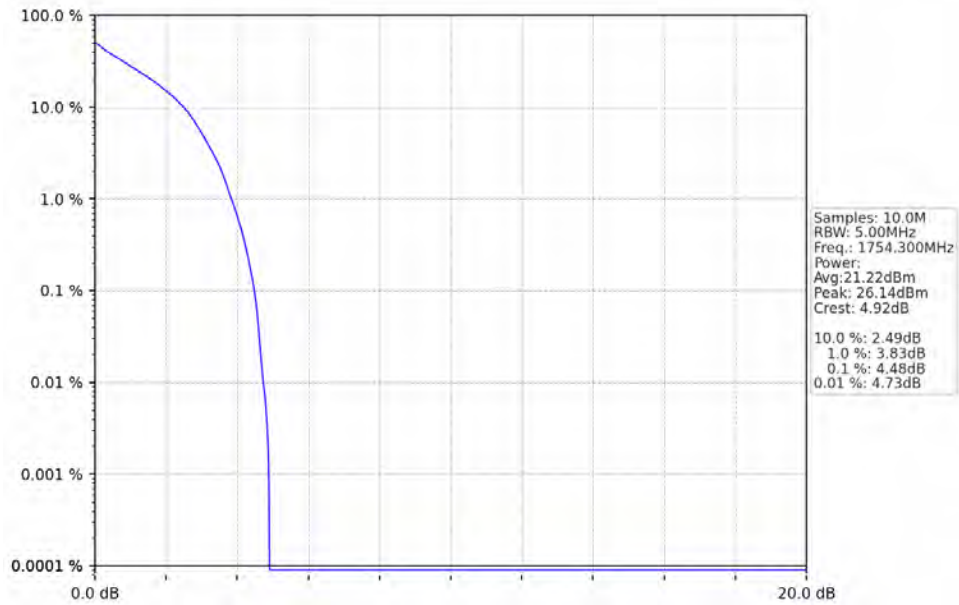
Band4 1.4MHz QPSK HCH 1754.3MHz RB 6 0 NTV
