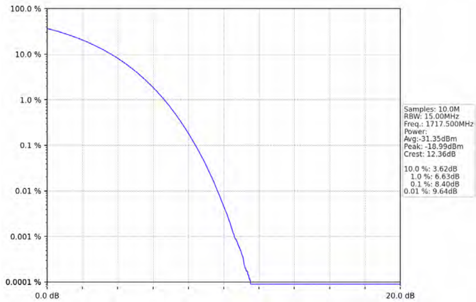
Band4 15MHz 16QAM LCH 1717.5MHz RB 27 0 NTNV
