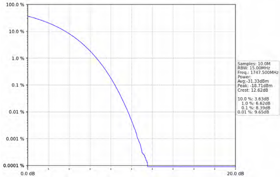
Band4 15MHz QPSK HCH 1747.5MHz RB 75 0 NTNV
