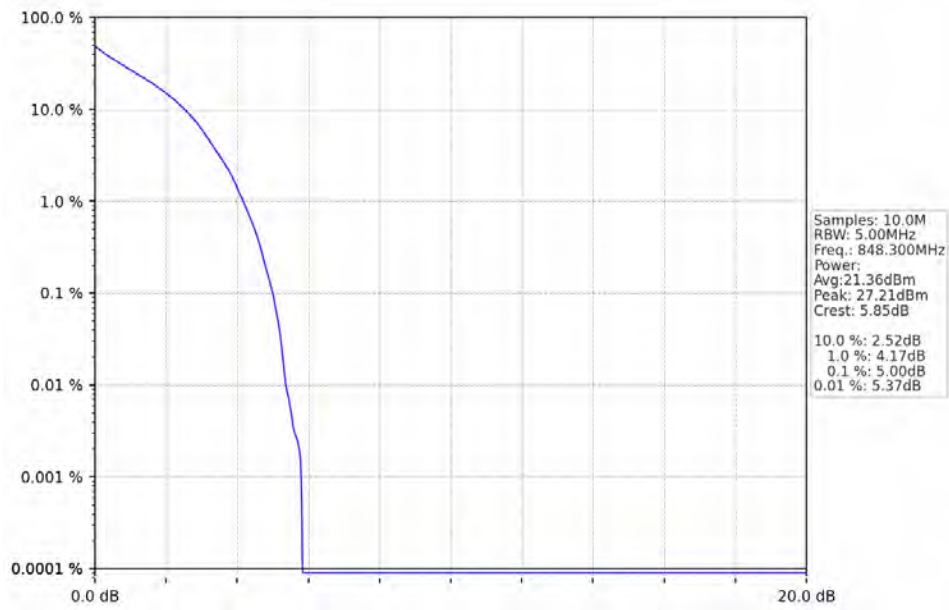
Band5_1.4MHz_QPSK_HCH_848.3MHz_RB_6_0_NTNV
