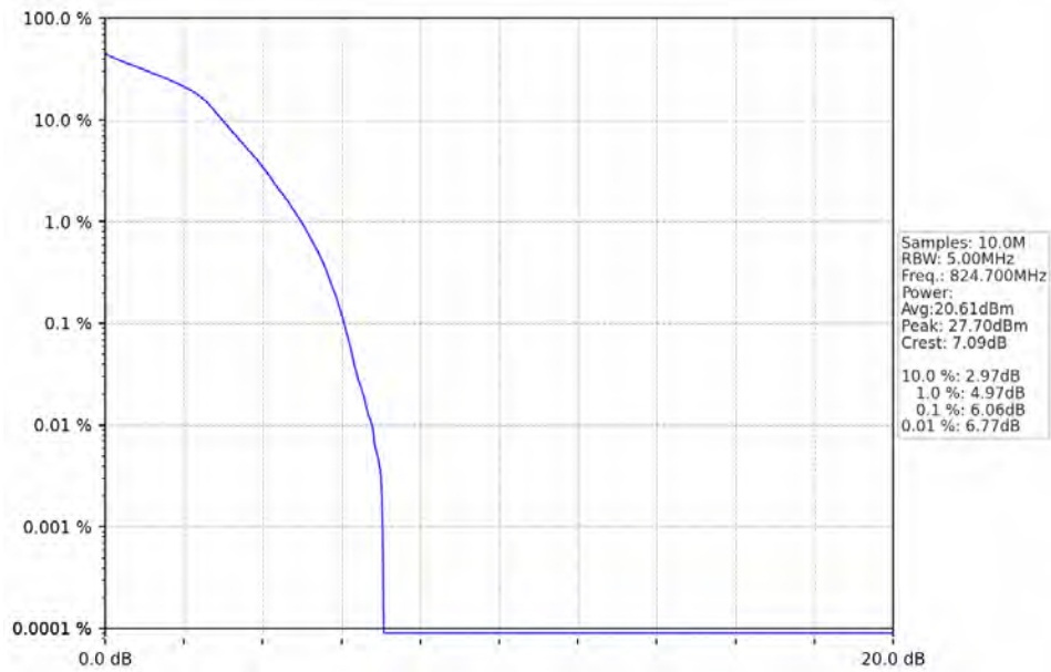
Band5_1.4MHz_16QAM_LCH_824.7MHz_RB_6_0_NTNV
