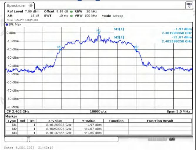
pi/4DQPSK_2-DH5_Channel 0
