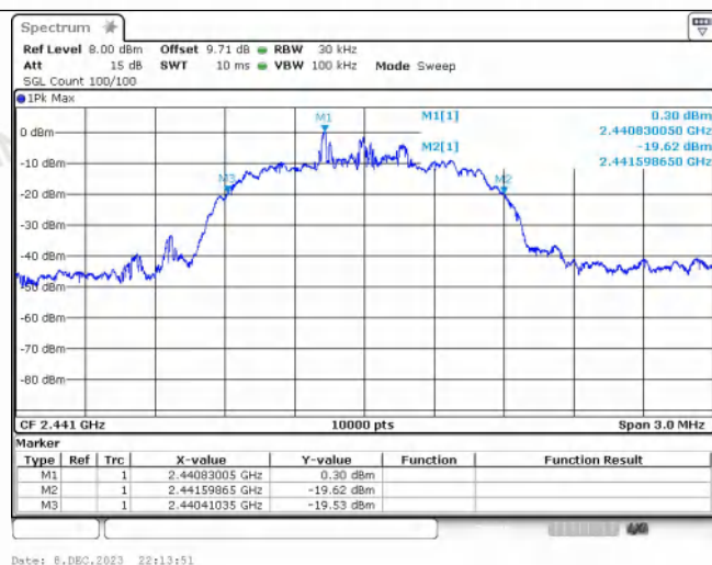
8DPSK_3-DH5_Channel 39
