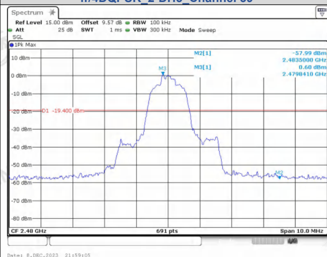
Out Of Band Emission π/4DQPSK_2-DH5_Channel 78
