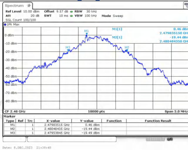
GFSK_DH5_Channel 78
