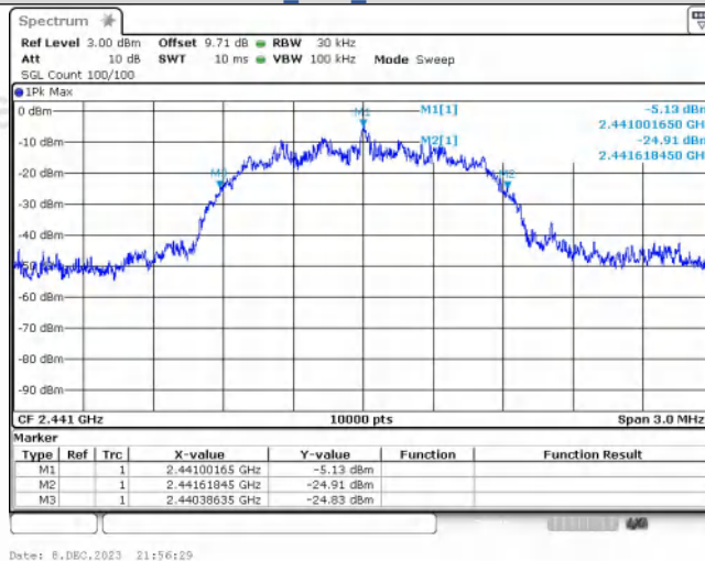
pi/4DQPSK_2-DH5_Channel 39
