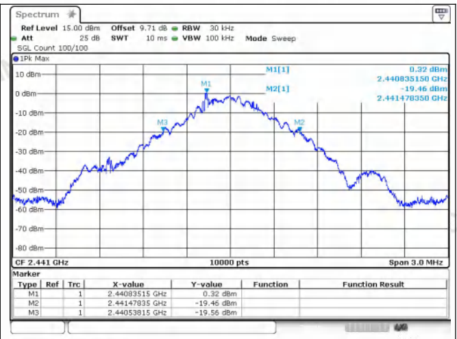
GFSK_DH5_Channel 39
