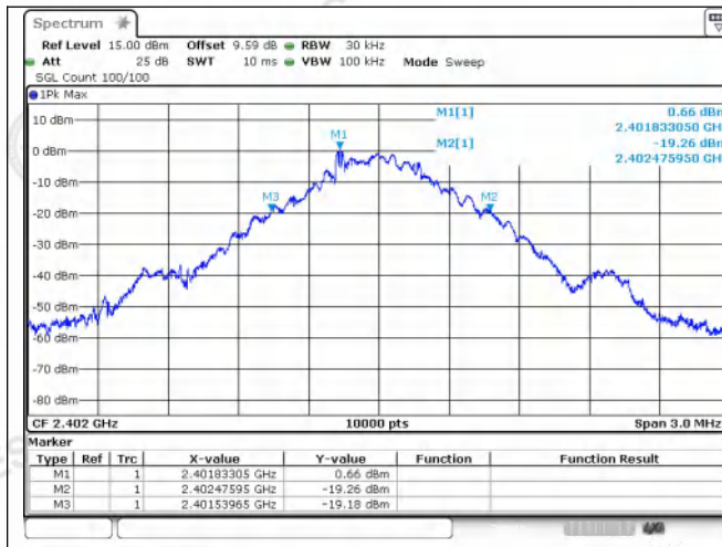
GFSK_DH5_Channel 0
