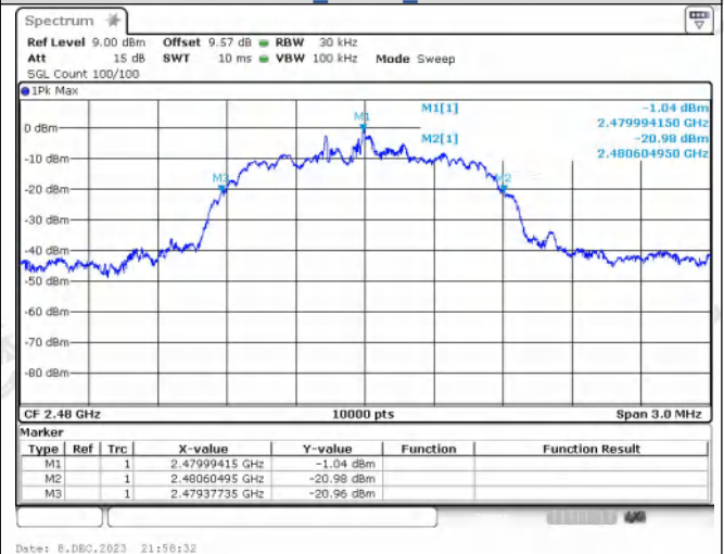
pi/4DQPSK_2-DH5_Channel 78
