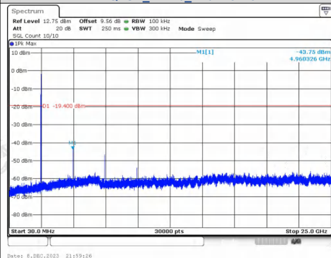
Spurious Emission π/4DQPSK_2-DH5_Channel 78
