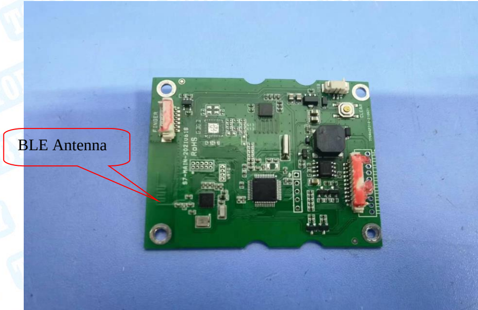
Photo 15 Appearance of PCB
