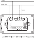
Live & Neutral wire (Neutral wire Required)
