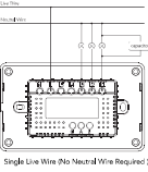
Single Live Wire (No Neutral Wire Required)
