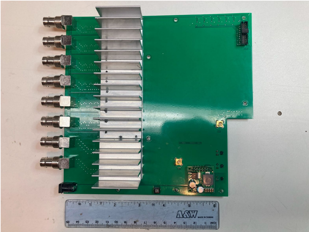
MAIN PRINTED CIRCUIT BOARD
